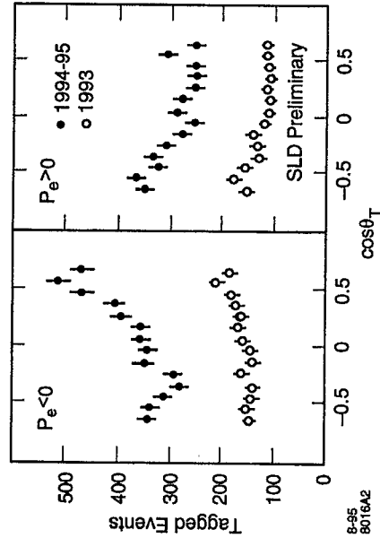
Fig. 2. Forward-backward asymmetry for tagged b events.
