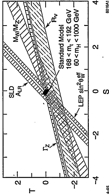
Fig. 1. Electroweak data in the S, T plane.
