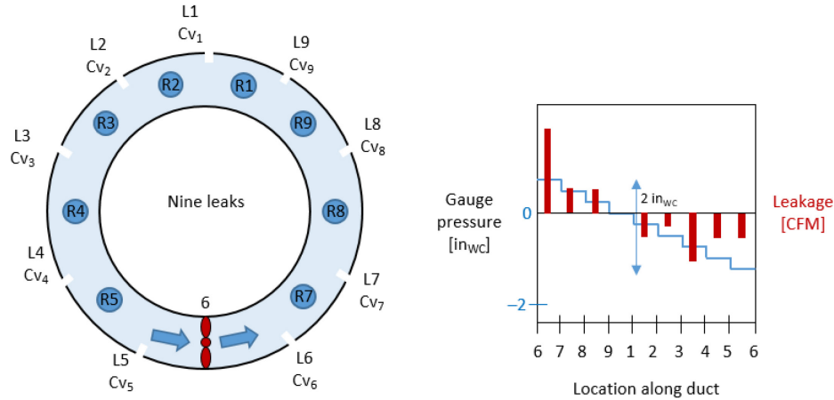
Figure 17. Circular duct with fan, a series of discrete flow resistances (component pressure drops), and an equal number of leakage locations of varying size.
