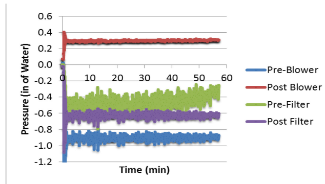
Figure 4. Gauge pressures of the first generation prototype during operation.
