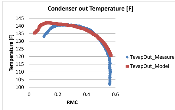
Figure 41. Measured and predicted condenser exit air temperatures.
