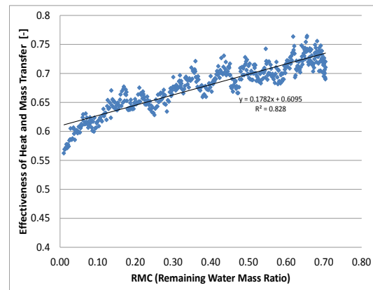
Figure 31. Heat and mass effectiveness of first generation drum.
