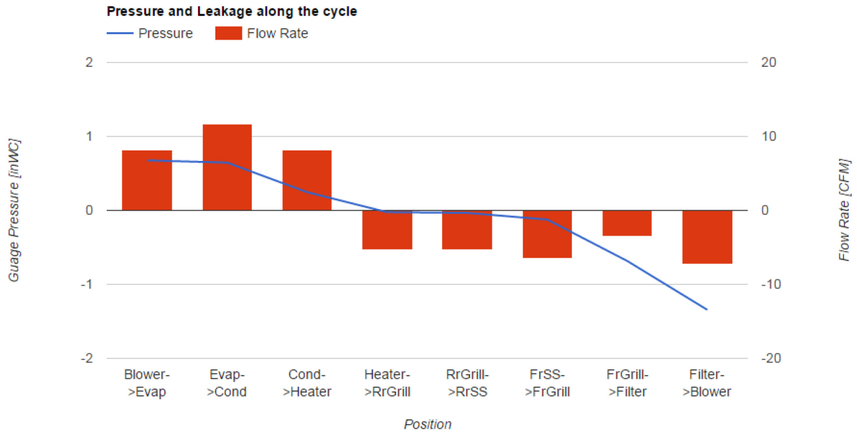
Figure 19. Example output of the HTML-based leakage calculator, showing pressure profile and leakage rates for a given set of measured C_v s and \Delta P s relevant to the second generation HPCD prototype.
