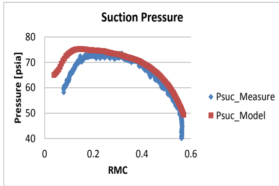
Figure 36. Measured and predicted suction pressures.
