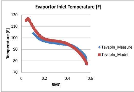
Figure 39. Measured and predicted evaporator inlet air temperatures.
