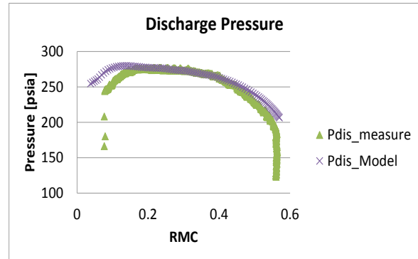
Figure 37. Measured and predicted discharge pressures.
