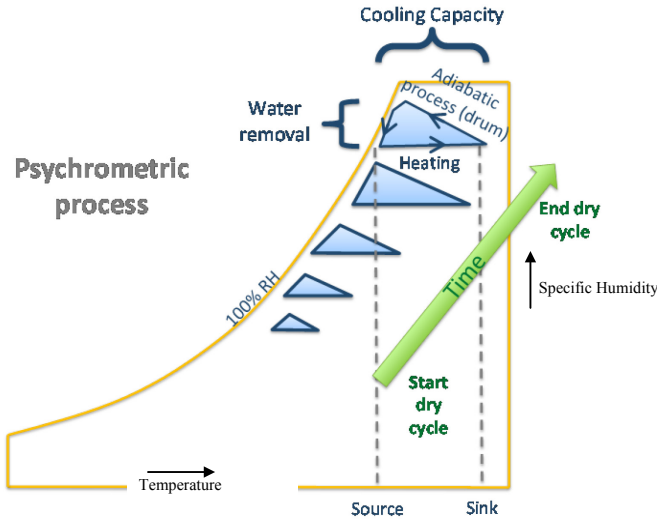
Figure 27. Transient clothes drying process in a psychrometric chart.
