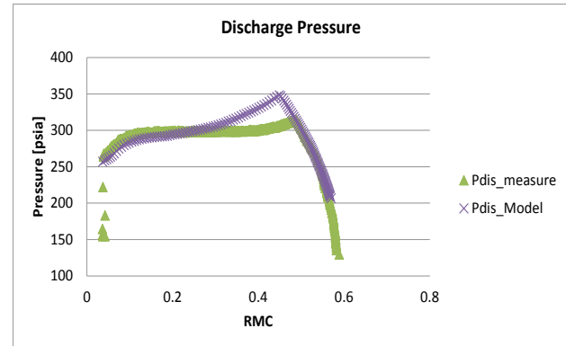
Figure 43. Measured and predicted discharge pressures with running heater for 10 minutes.
