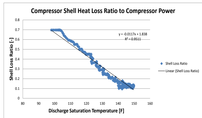
Figure 33. Compressor shell-heat loss ratio to compressor power.
