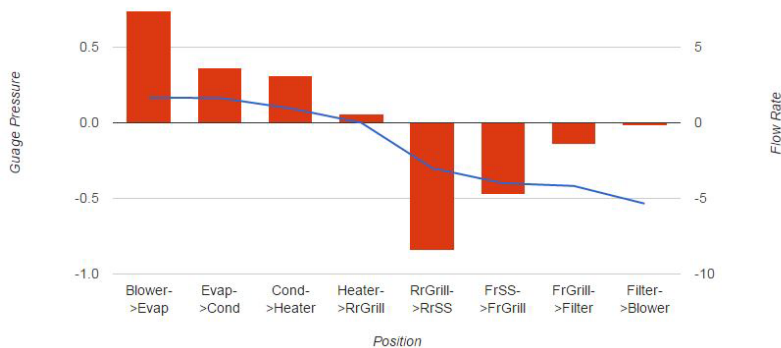
Figure 35. Local static pressures and leakage flow rates.
