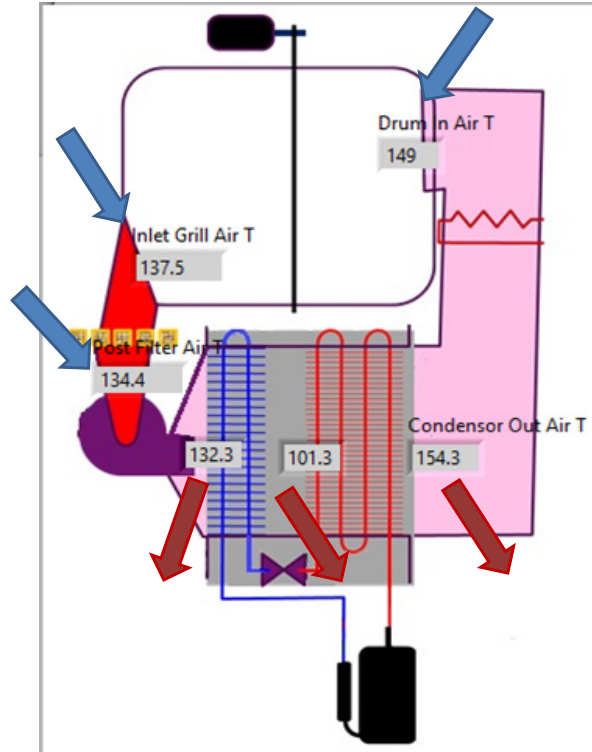
Figure 29. System diagram of GE heat pump clothes dryer.
