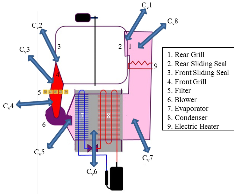
Figure 18. Flow-restriction components and leakage segments of the second generation prototype dryer.
