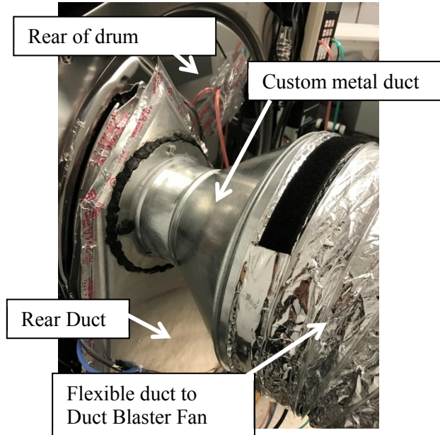
Figure 10. Custom metal duct to interface Duct Blaster to HPCD for leakage testing.
