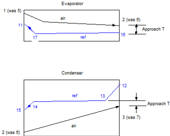
Figure 48. Definition of fixed approach temperatures used in EES model. Refrigerant state points are shown in blue, and psychrometric state points in black, with first and second generation designations shown.
