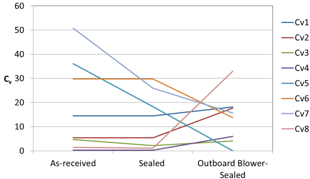
Figure 20. Change in C_v at all leakage locations in airflow path due to sealing activities.
