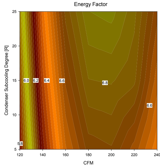
Figure 45. EF changing with airflow rate and condenser subcooling degree.
