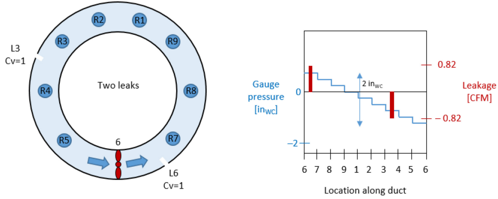
Figure 16. Circular duct with fan, a series of discrete pressure drops, and two small leaks.
