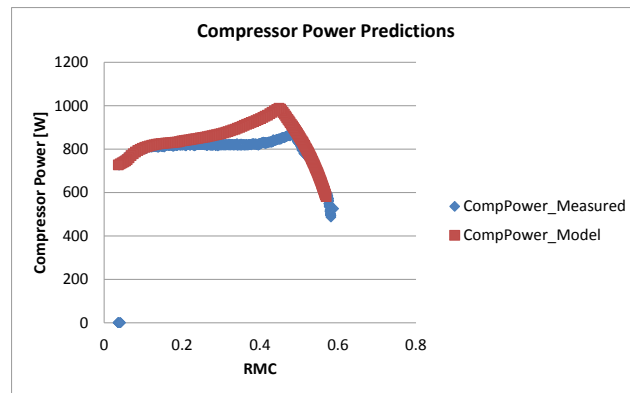
Figure 44. Measured and predicted compressor powers with running heater for 10 minutes.
