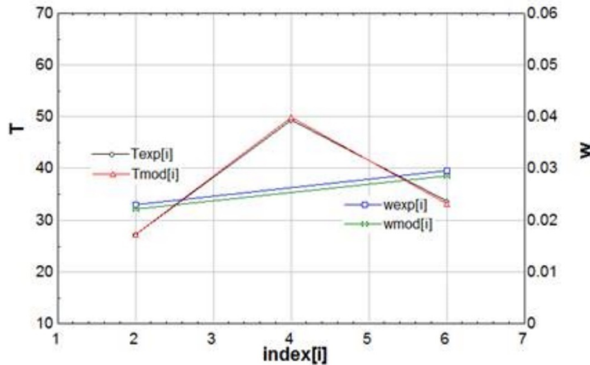
Figure 49. The EES model was calibrated to match three key state points (2, 4, and 6) against a single baseline experimental CEF trial
