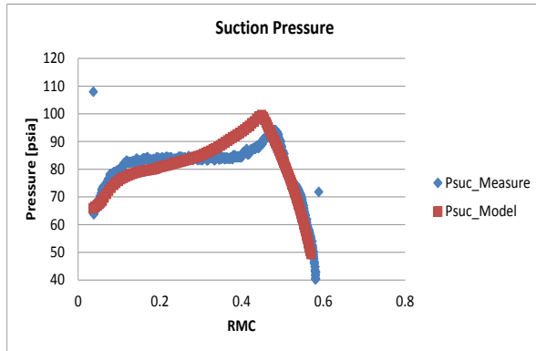
Figure 42. Measured and predicted suction pressures with running heater for 10 minutes.
