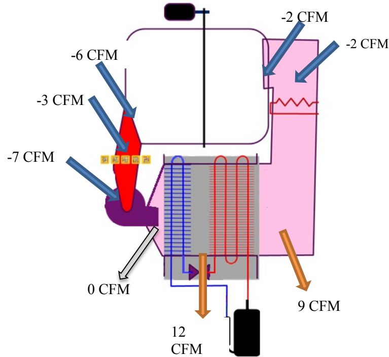
Figure 22. The baseline leakage of the outboard blower setup.
