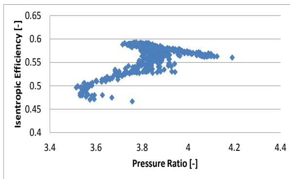
Figure 32. Compressor isentropic efficiency.
