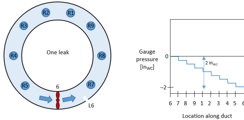
Figure 15. Circular duct with fan, a series of discrete pressure drops, and one small leak.
