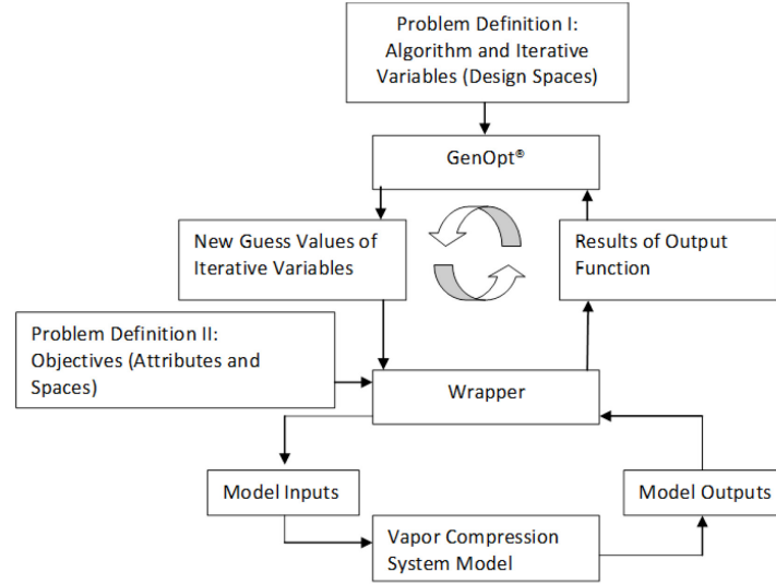
Figure 23. GenOpt Optimization Wrapper to a Vapor Compression System Model.
