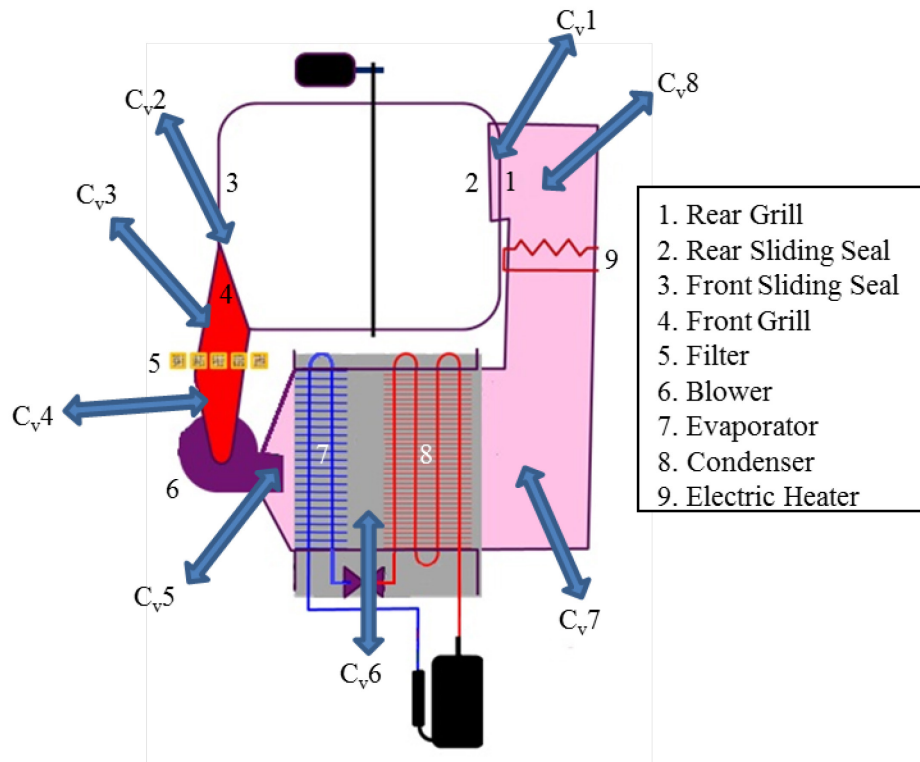
Figure 11. Schematic of HPCD air loop showing air leakage locations as C_v\# and components that can produce pressure drops in airflow path.
