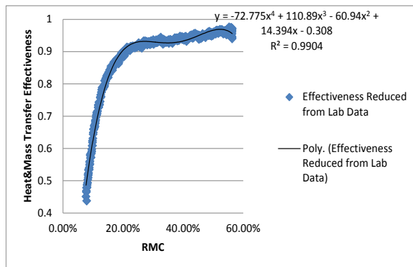
Figure 30. Heat and mass effectiveness of second generation drum.
