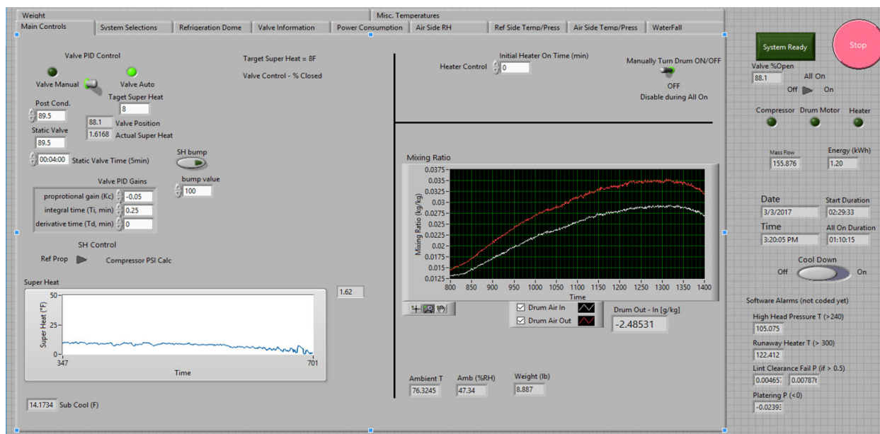
Figure 3. The main tab of the HPCD control program is used to monitor and control EXV position and superheat, as well as monitor the absolute moisture of the air coming into and out of the drum.
