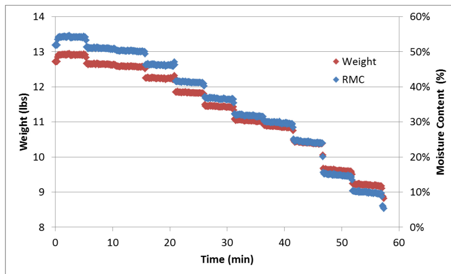
Figure 5. Load weight and RMC over time for the first generation prototype.
