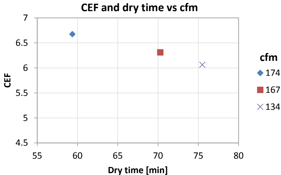
Figure 9. CEF and dry time results from different airflow rates.
