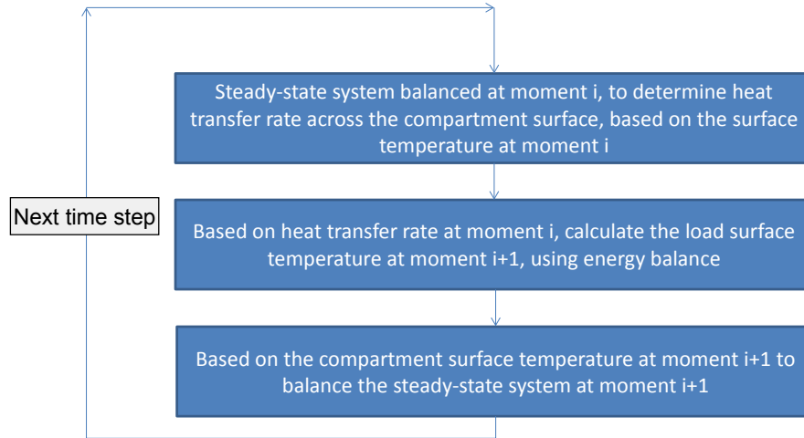
Figure 28. Quasi-steady-state time step.
