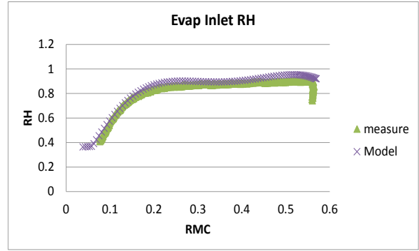
Figure 40. Measured and predicted evaporator inlet air relative humidities.
