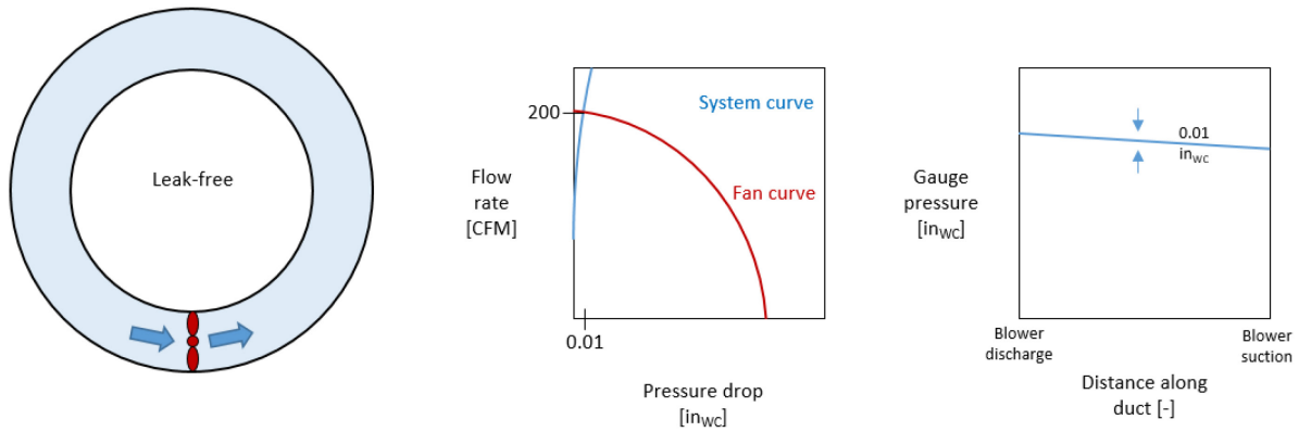
Figure 13. Leak-free circular duct with fan and negligible pressure drop.
