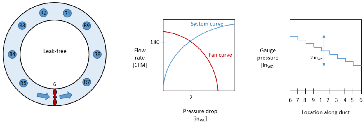
Figure 14. Leak-free circular duct with fan and a series of discrete non-negligible pressure drops.
