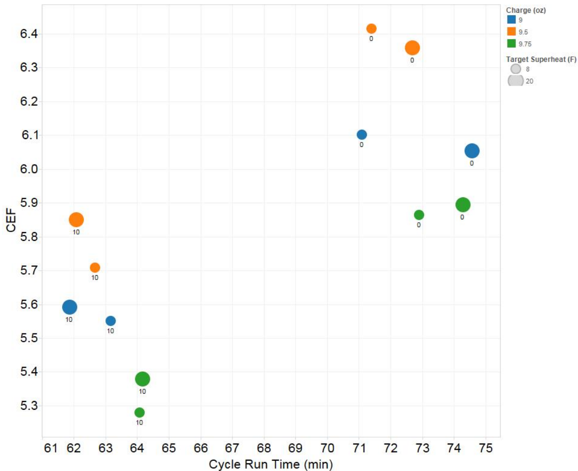
Figure 8. Graphical representation of test matrix results for optimizing charge, superheat and heater on time.
