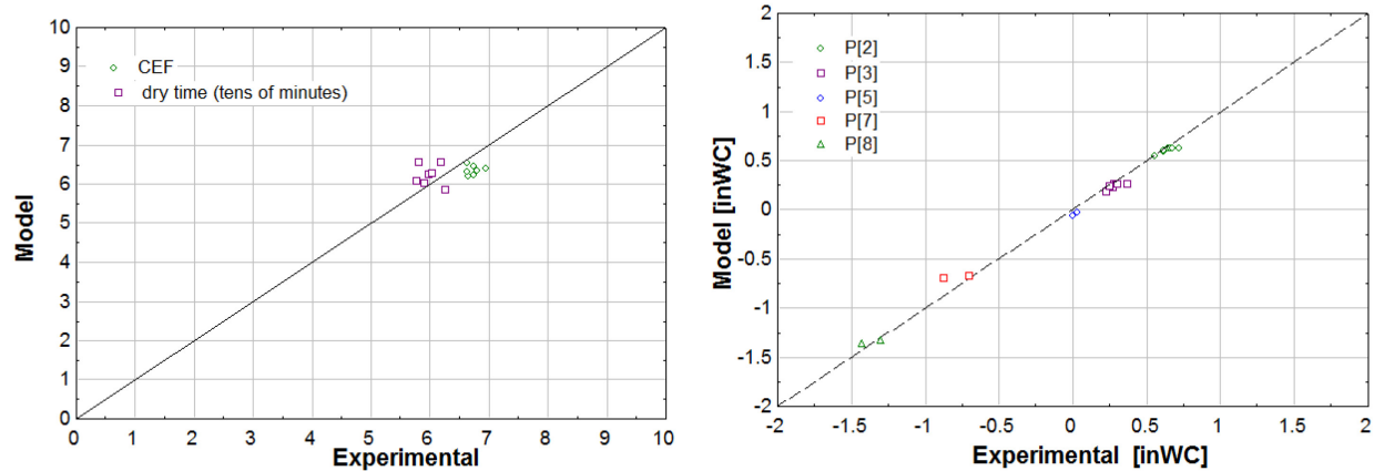
Figure 50. Experimental validation of HPCD system model CEF and dry time on left, and gauge pressures on right.
