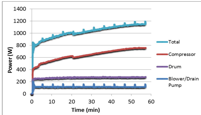
Figure 6. Power consumption of the first generation dryer over time.
