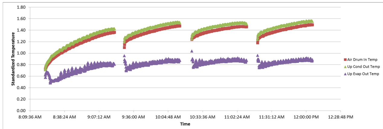
Figure 7. Temperatures for four back-to-back cycles of first generation prototype.
