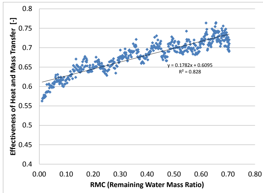
Figure 24. Drum heat and mass transfer effectiveness as a function of RMC for one run of the first generation HPCD prototype.
