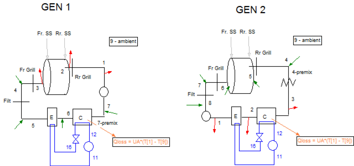
Figure 46. First generation (pressurized drum) and second generation (negative pressure drum) state points in EES model. Note SS = sliding seal.
