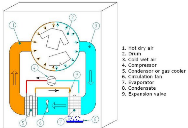
Figure 26. Schematics of a heat pump clothes dryer.
