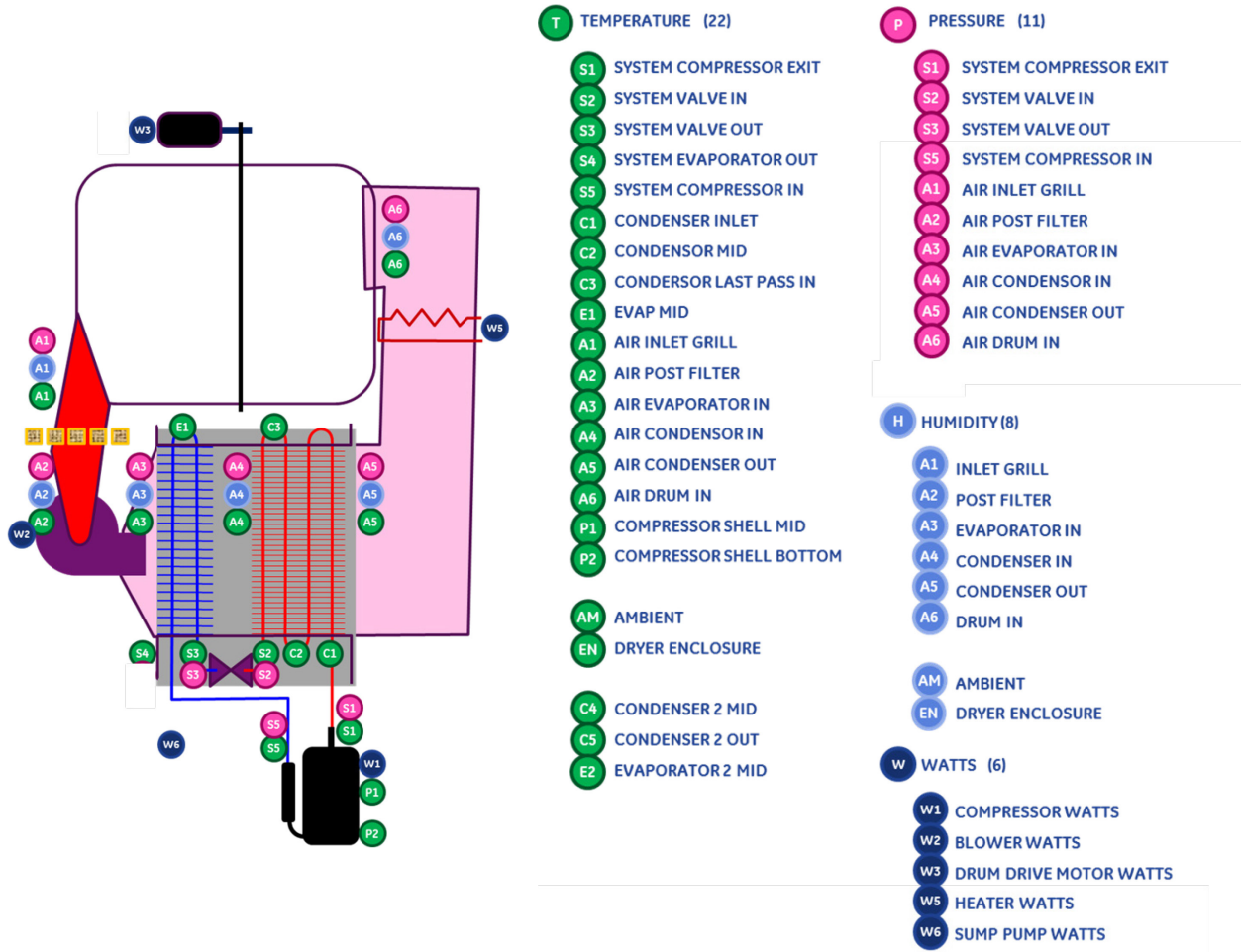
Figure 2. Schematic of second generation HPCD prototype with type and locations of all sensors.
