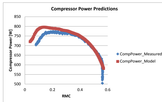
Figure 38. Measured and predicted compressor powers.
