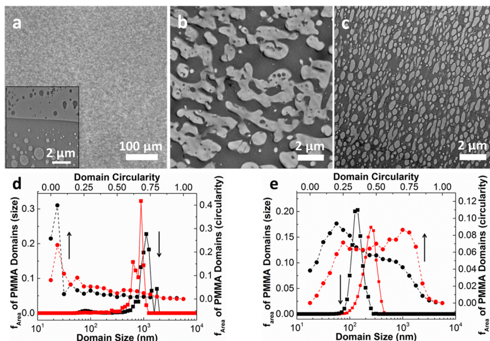
Figure 6. Images of morphology after annealing of 44:56 PS:PMMA samples for 4 days at 160 °C, for comparison to as-cast structures shown in Figures 2a,b,d. (a) Optical micrograph of 0% JP blend (inset: TEM micrograph of film cross section) and TEM micrographs of (b) 8 and (c) 20 vol % JP. Area-weighted distributions of PMMA domain size (solid lines) and circularity (dotted lines) for both as-cast (black) and annealed (red) for (d) 8 and (e) 20 vol % SBM JP.
