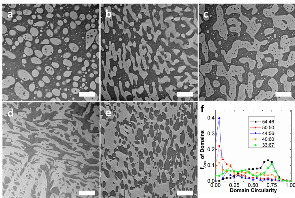
Figure 4. TEM micrographs demonstrating the change in domain shape of PS/PMMA blends with 8 vol % SBM JPs in response to changes in blend composition: (a) 54:46, (b) 50:50, (c) 44:56, (d) 40:60, and (e) 33:67 PS:PMMA. Scale bars represent 2 \mu\text{m} . (f) Histogram plot of the area-weighted fraction of dispersed domains as a function of their circularity, as determined by image analysis.
