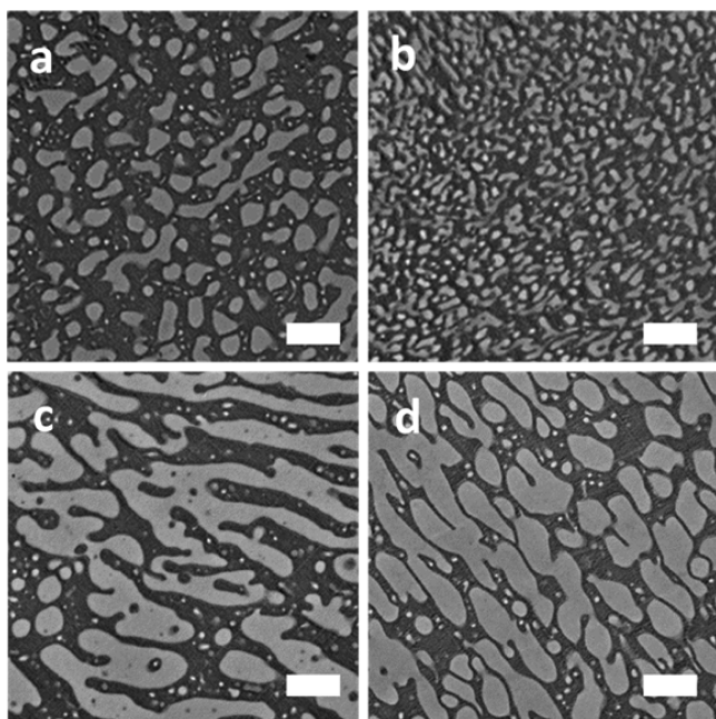
Figure 5. TEM micrographs demonstrating change in domain shape of PS/PMMA blends with 20 vol % SBM JPs in response to changes in blend composition: (a) 47:53, (b) 44:56, (c) 40:60, (d) 33:67 PS:PMMA. Scale bars represent 1 \mu\text{m} .
