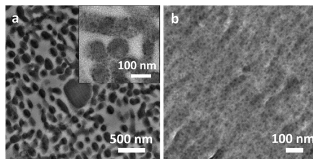
Figure 7. Films with higher and lower molecular weight matrix homopolymers. (a) TEM micrographs of 50:50 PS (127 kg/mol):PMMA (120 kg/mol) + 20 vol % SBM JP (inset: detail showing JP assembly inside PS domains, indicative of preferential interaction of the particles with PS). (b) TEM micrograph showing a phase-mixed structure in 50:50 PS (3.2 kg/mol):PMMA (5.0 kg/mol) + 20 vol % SBM JP, featuring increased core-to-core distance of about 40 nm.
