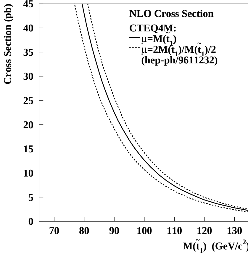
Figure 1.1: The theoretical next-to-leading order cross section for p\bar{p} \rightarrow \tilde{t}_1\tilde{t}_1 at \sqrt{s} = 1.8 TeV with CTEQ4M using PROSPINO
