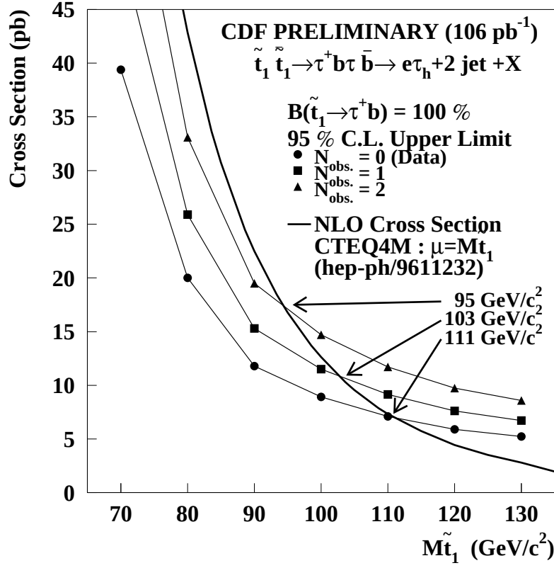
Figure 5.2: 95% confidence level on upper limit for cross section for \tilde{t}_1 \tilde{t}_1^* \rightarrow \tau^+ b \tau^- \bar{b} along with the theoretical calculation in the case of the observed events number = 0, 1, 2
