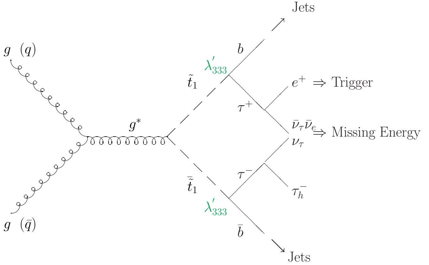
Figure 1.3: The Feynman diagrams for scalar top quark pair-production by R -parity \lambda'_{333} coupling violating decay
