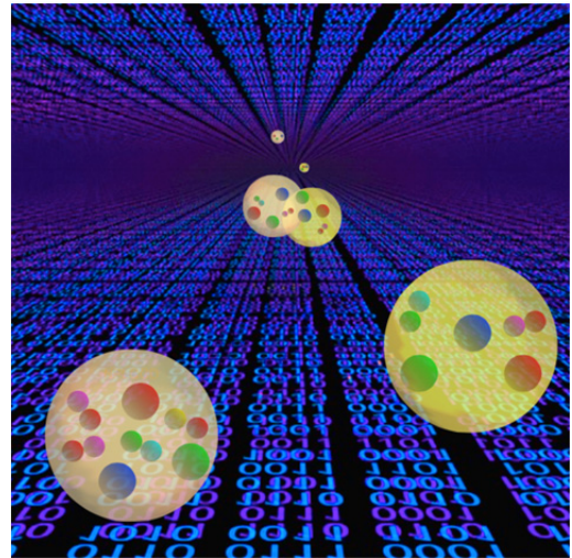
Figure 2. A cartoon of nucleon-nucleon scattering. Image reproduced with permission from Martin Savage (INT).
