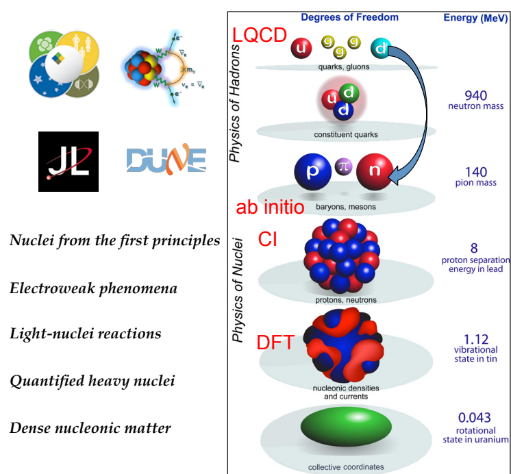
Figure 3-15. Left: Case studies of the NS&R exascale program. Right: The basic elements that atomic nuclei are made of depend on the energy of the experimental probe and the distance scale. The building blocks of QCD are quarks and gluons, which form the mesons and baryons. In low-energy nuclear physics experiments, nuclei can be well described in terms of individual protons and neutrons, their densities and currents, or collective coordinates describing rotations and vibrations of the nucleus as a whole. Major theoretical approaches to the nuclear many-body problem (lattice QCD, ab initio methods, configuration interaction techniques, nuclear DFT, and collective models) are marked at different resolution scales. (Image reproduced with permission from Witke Nazarewicz; available in Bertsch et al. 2007.)
