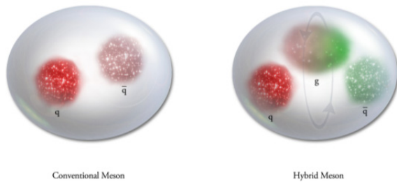
Figure 3. A cartoon showing the naive structure of a conventional meson (left) and of a hybrid meson explicitly involving excitations of the glue. Image reproduced with permission from Robert Edwards (JLab).
