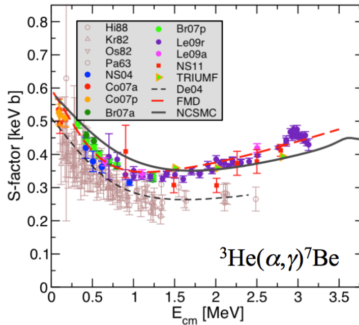
Figure 3-19. Capture of ^3\text{He} by alpha particles to form ^7\text{Be} . Ab initio techniques make it possible to calculate low-energy reactions, and exascale computing resources will enable the calculation of many important processes that are difficult to measure in the laboratory. (Image reproduced with permission from Sofia Quaglioni; available in Doherty et al. 2016.)
