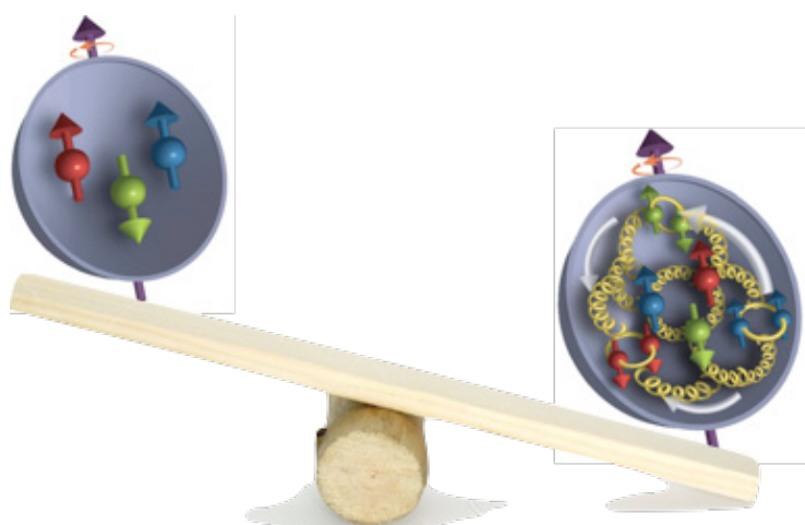
Figure 3-28. Lattice QCD calculations of the gluonic structure of the proton that are anticipated in the exascale era will support and complement an EIC experimental program envisioned as the future of QCD research in the United States. (Figure reproduced with permission from David Richards.)
