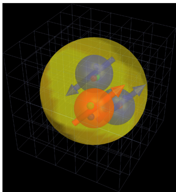
Figure 1. The magnetic moments and polarizabilities of light nuclei are now being calculated with lattice QCD. (Image reproduced with permission from William Detmold.)
