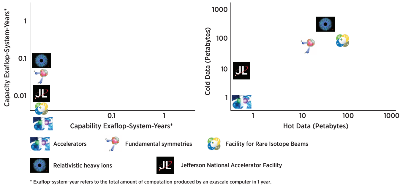
Figure 3-14. The capability and capacity computing resource requirements (left panel) and the hot and cold data requirements (right panel) in 2025 to accomplish the objectives of the NP Experiment and Data program.
