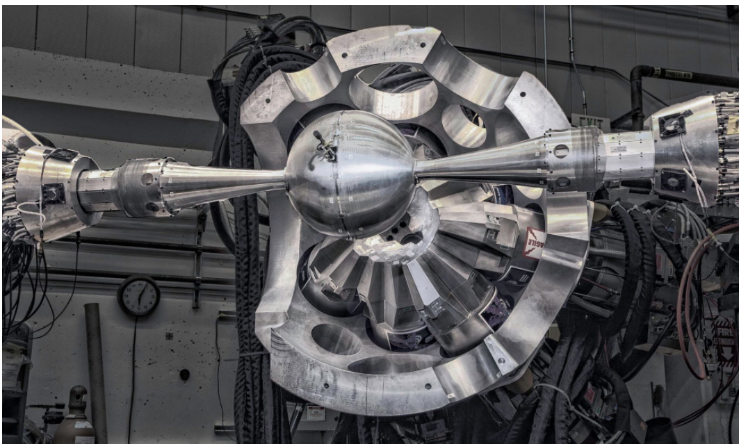
Figure 3-10. GRETA is the predecessor for the GRETA gamma-ray tracking detector array. The construction of GRETA, a full 4\pi coverage device, with increased rate requirements, coupled with the need for real-time processing, requires significant I/O, CPU, memory, and storage resources. (Image by Kevin Bailey of Argonne National Laboratory; reproduced with permission from Shaofei Zhu.)
