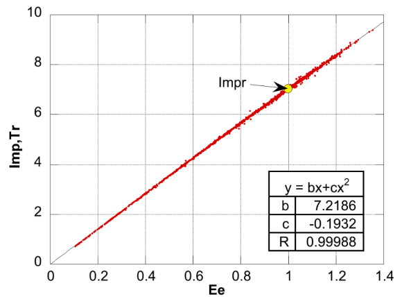
Fig. 4. Determination of I_{mpr} , C_0 and C_1
