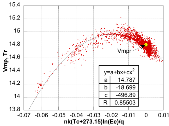
Fig. 5. Determination of V_{mpr} , C_2 and C_3 .
