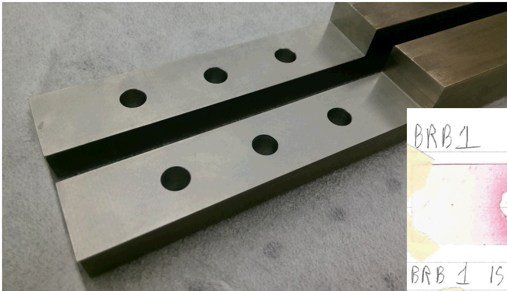
Classic Brake-Reuß Beam (BRB)
