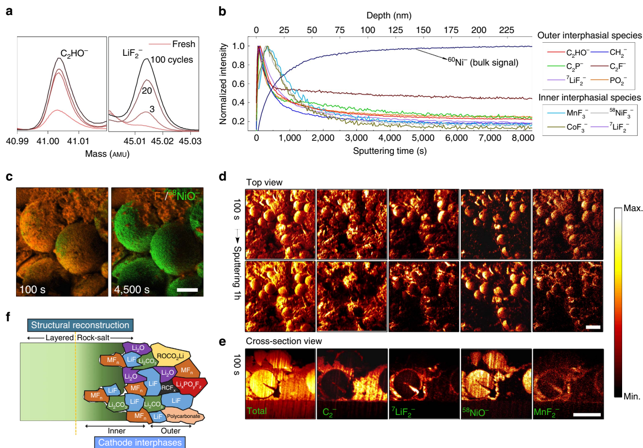
Figure 1 | Localization and visualization of interphases at the surface of cycled \text{LiNi}_{0.7}\text{Mn}_{0.15}\text{Co}_{0.15}\text{O}_2 . (a) TOF-SIMS spectra of \text{C}_2\text{HO}^- and ^7\text{LiF}_2^- integrated over 1,000 s of \text{Cs}^+ sputtering (10 s sampling step) on \text{LiNi}_{0.7}\text{Mn}_{0.15}\text{Co}_{0.15}\text{O}_2 composite electrodes after battery operation at room temperature, representative of the evolution of organic and inorganic interphasial species as a function of cycles. (b) Normalized (to maximum) depth profiling of several secondary ion fragments of interest at the cycled \text{LiNi}_{0.7}\text{Mn}_{0.15}\text{Co}_{0.15}\text{O}_2 surface. Depth is calculated based on the calibrated \text{Cs}^+ sputtering rate of \sim 0.03 \text{ nm s}^{-1} for the active material (Supplementary Fig. 1). (c–e) TOF-SIMS chemical mapping (burst alignment mode) on cycled \text{LiNi}_{0.7}\text{Mn}_{0.15}\text{Co}_{0.15}\text{O}_2 electrodes. (c) Illustrative maps of \text{F}^- and ^{58}\text{NiO}^- before and after intensive \text{Cs}^+ sputtering, depicting the interphases on the composite electrode of secondary particles, additive carbon and polymeric binder (100 s shallow milling was applied in order to reduce possible contamination, such as adventitious chemisorbed carbon). Scale bar, 10 \mu\text{m} . (d,e) Comparative chemical mapping of several fragments, unraveling the complex interphases on the electrode. (d) Shows top views collected after 100 s and 1 h \text{Cs}^+ etching, while e is taken from the cross-sectional perspective. From the left to right, the secondary ions of interest are, respectively, 'total', \text{C}_2^- , ^7\text{LiF}_2^- , ^{58}\text{NiO}^- and \text{MnF}_2^- . Scale bars, 20 \mu\text{m} in both d,e. (f) A schematic diagram of the microstructure and chemical composition of surface degradation products at the surface of \text{LiNi}_{0.7}\text{Mn}_{0.15}\text{Co}_{0.15}\text{O}_2 . The size of regions is not drawn to scale.
