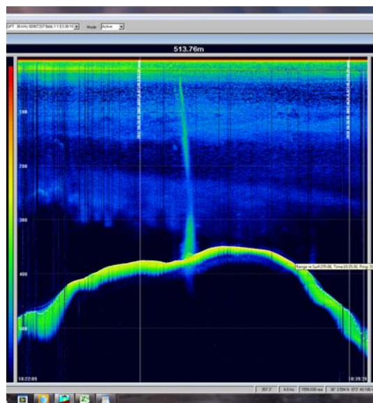
Figure A5. Raw EK60 record of a gas plume emanating from the seafloor at ~375 m water depth near Baltimore Canyon as recorded during the R/V Sharp cruise. Although the bubbles clearly continue to 40 m or shallower within the water column, the bubbles should by then have lost all of their methane to the surrounding waters.
