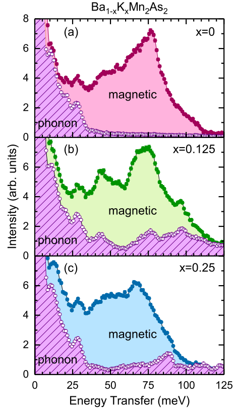
Figure 8: High-angle spectra (empty symbols) and scaled low-angle spectra (solid symbols) at E_i = 144.7 meV for (a) x = 0 , (b) 0.125, and (c) 0.25. The shaded region corresponds to the estimated magnetic scattering spectrum S_{\text{mag}}(E) and the hatched shaded area is K S_{\text{high}}(E) \approx S_{\text{ph}}(E) + B(E) .
