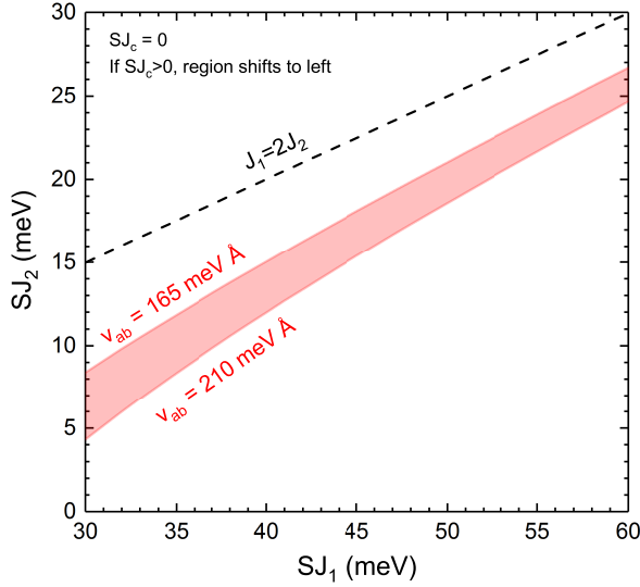
Figure 10: Region of SJ_1 - SJ_2 parameter space delineated by boundaries of v_{ab} from 165 to 210 meV Å with SJ_c = 0 is shown as the shaded region. For a G-type ground state, values of (SJ_1, SJ_2) above the dashed line correspond to the condition J_1 < 2J_2 and are not allowed.
