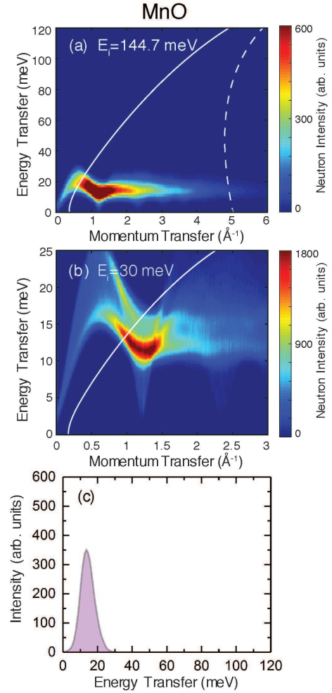
Figure 9: Calculations of the powder-averaged spin wave scattering from MnO. The full neutron intensity S(Q, E) is shown for an incident energy of (a) 144.7 meV and (b) 30 meV. The solid line denotes the kinematic limit near forward scattering ( 2\theta = 2.5 degrees) and the dashed line in panel (a) corresponds to a scattering angle of 2\theta = 35 degrees. Panel (c) shows the MnO spin wave spectrum obtained at E_i = 144.7 meV after averaging over the angle range in (a).
