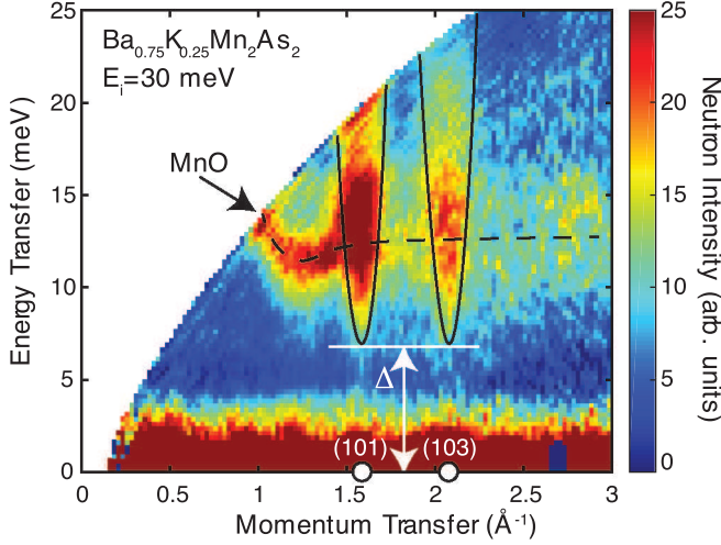
Figure 4: S(Q, E) profile of the \text{Ba}_{0.75}\text{K}_{0.25}\text{Mn}_2\text{As}_2 sample measured with E_i = 30 meV. Steeply dispersive excitations from Q_{(101)} and Q_{(103)} Bragg peaks are highlighted by the solid black outlines. It is evident that a well-defined energy gap ( \Delta ) exists which can be estimated visually to be about \Delta \approx 6 - 7 meV. The black dashed line highlights contributions of the spin wave scattering from MnO impurities that can be confirmed from MnO spin wave calculations shown in the Appendix.
