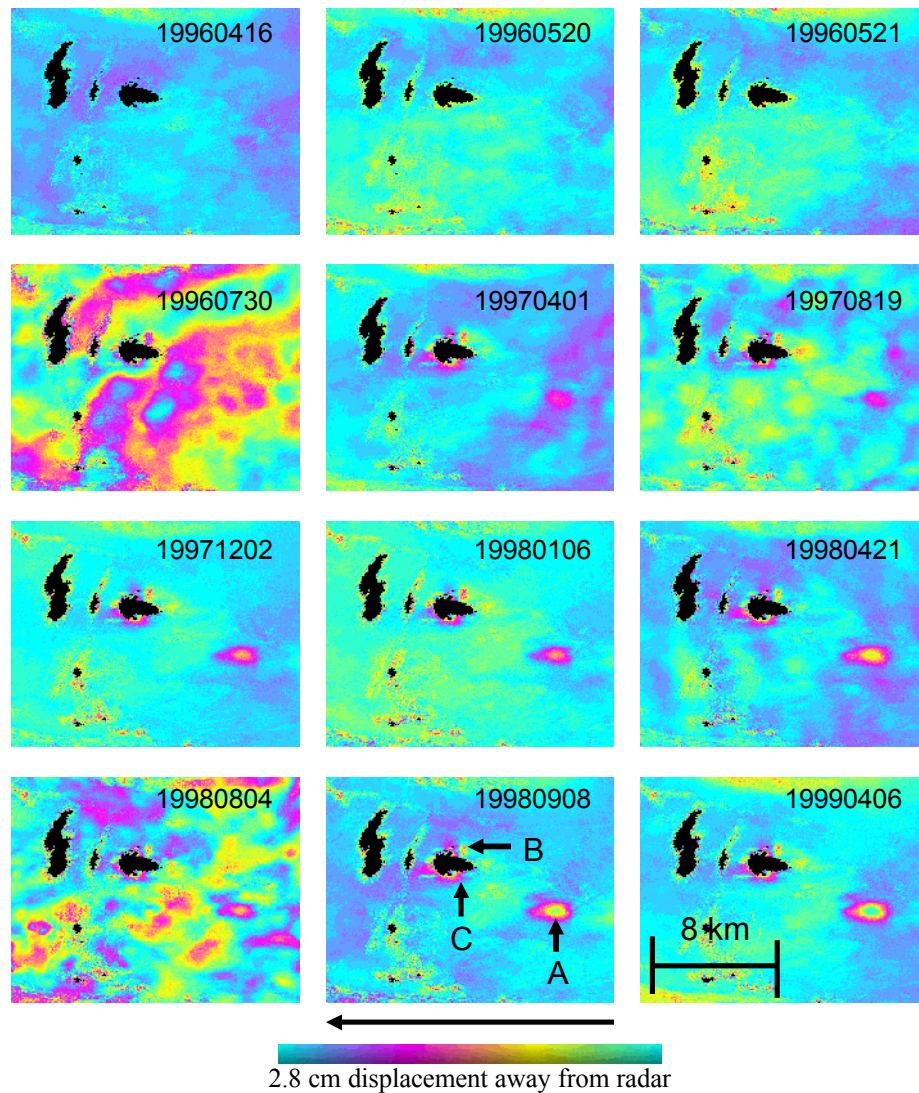
Figure 1. Maps of cumulative displacement since January 1, 1996 for Lop Nor. One cycle through color wheel represents 2.8 cm of radar line-of-sight displacement. The 19960730 and 19980804 images are noticeably afflicted with atmospheric artifacts.
