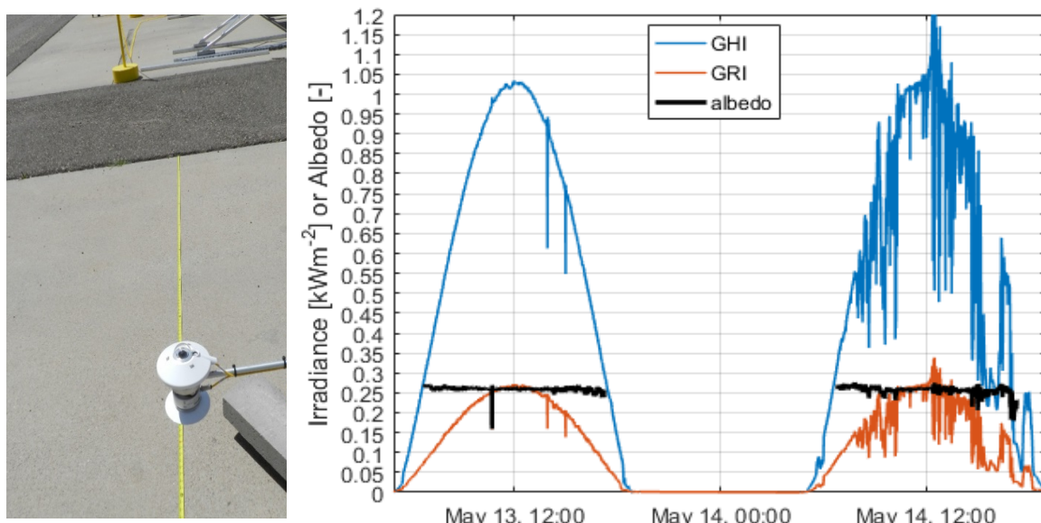
Figure 5: (Left) Albedometer setup on the natural surface. The yellow line is a tap measure used during installation and was not present during albedo measurements. (Right) Global horizontal irradiance (GHI), ground reflected irradiance (GRI), and albedo as measured by the albedometer.
