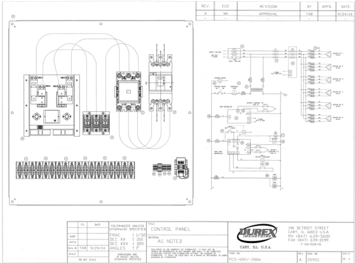
Figure 84. Process gas heater control panel schematic
