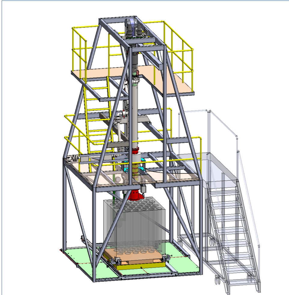
Figure 68. HOT test cell drill structure solid model
