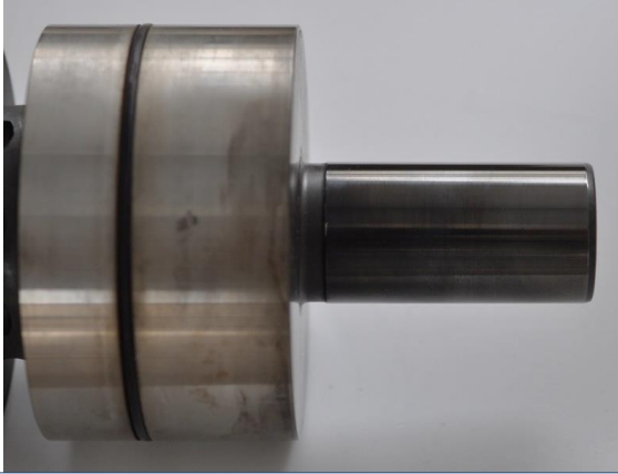
Figure 42. HT distributor performance after 54.5 cumulative feet
