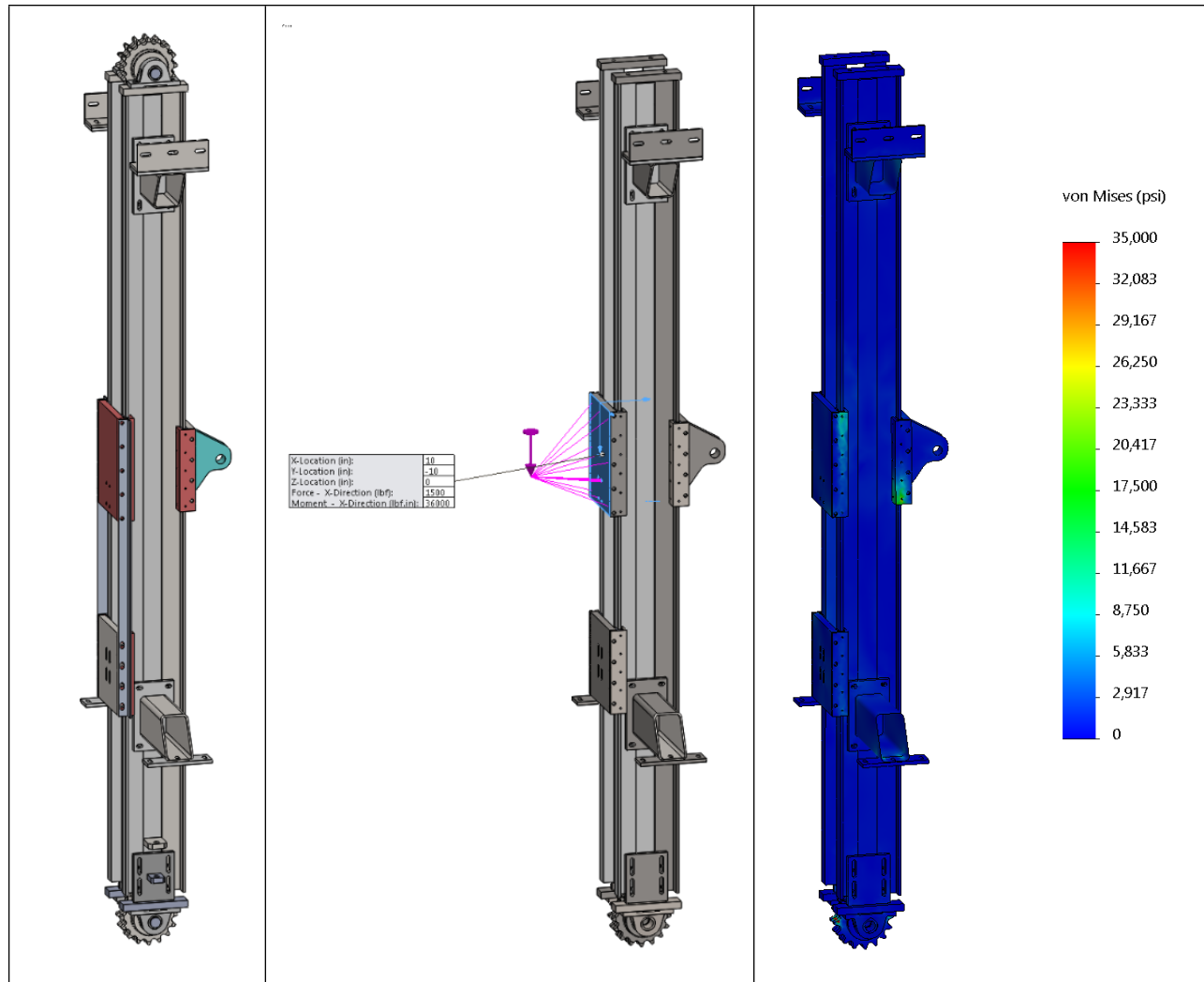
Figure 70. Mast design and stress analysis
