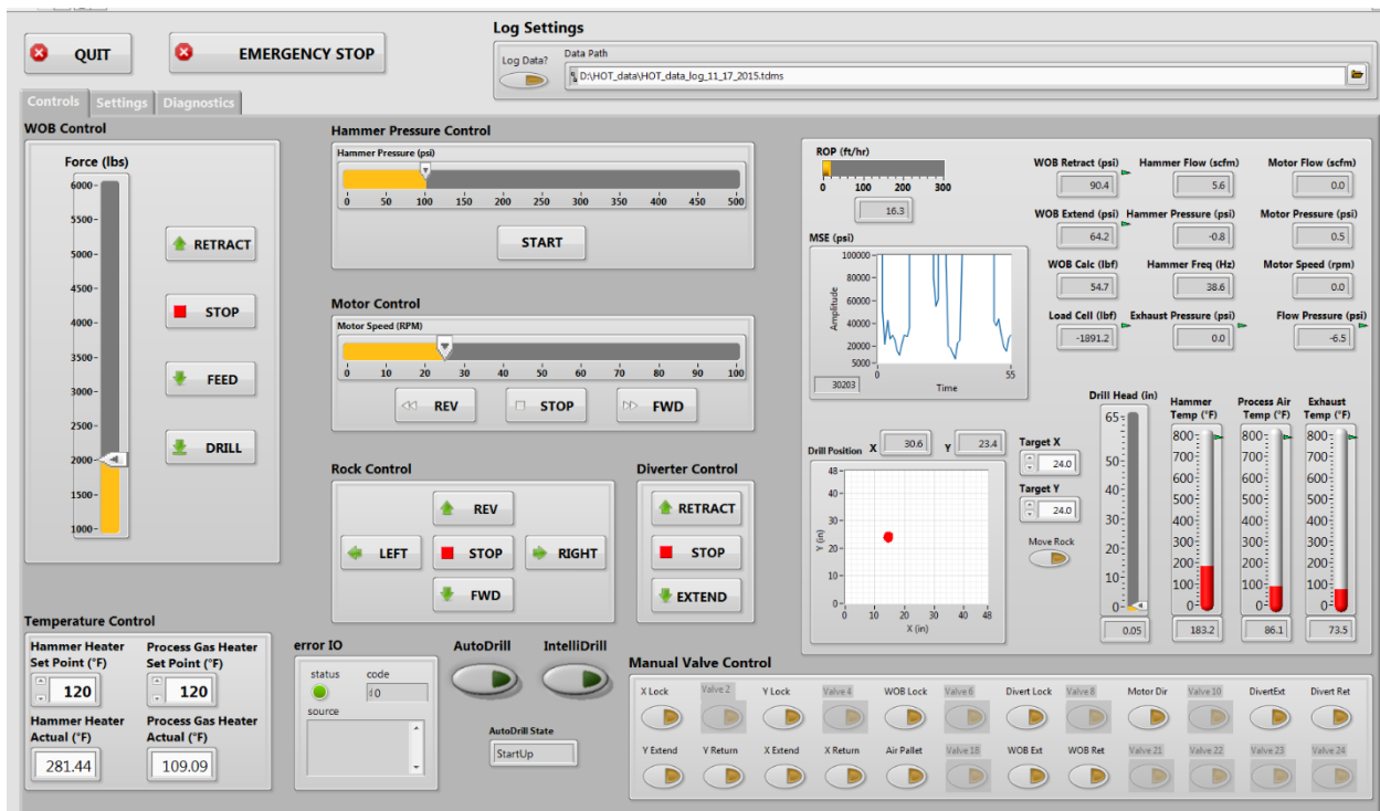
Figure 83. HOT control panel screen capture
