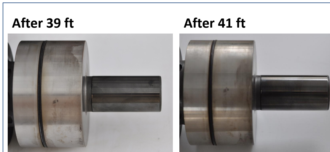
Figure 40. HT distributor performance continued from previous tests
