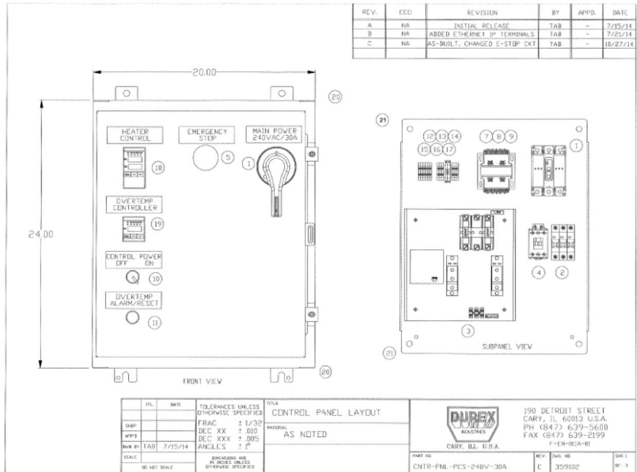
Figure 86. Heater/diverter control panel
