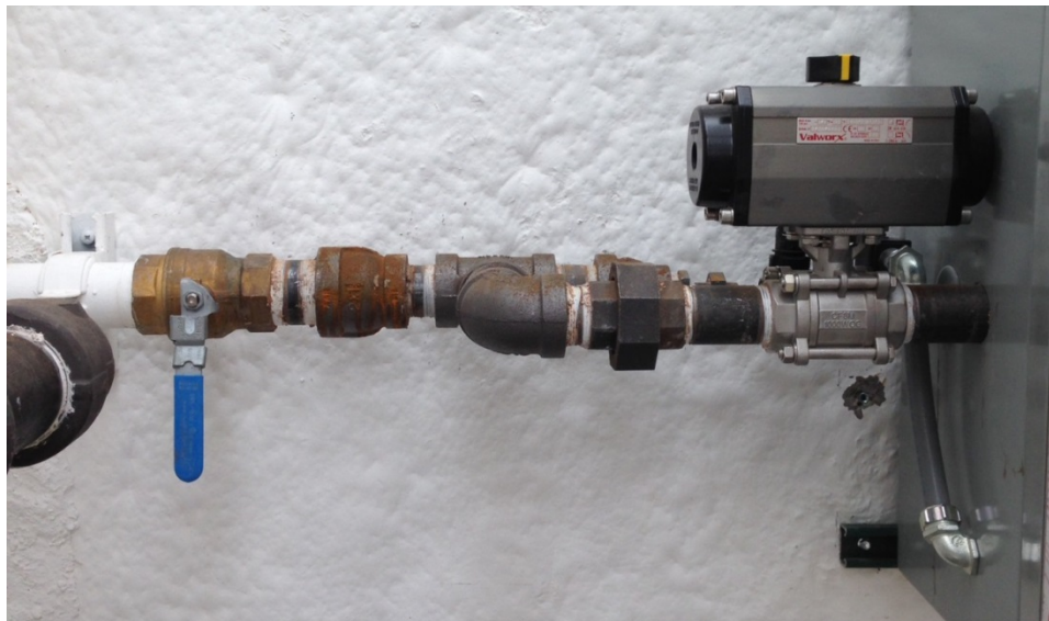
Figure 57. Control Box Entry (2" pipe to 1 1/2" reduction)
