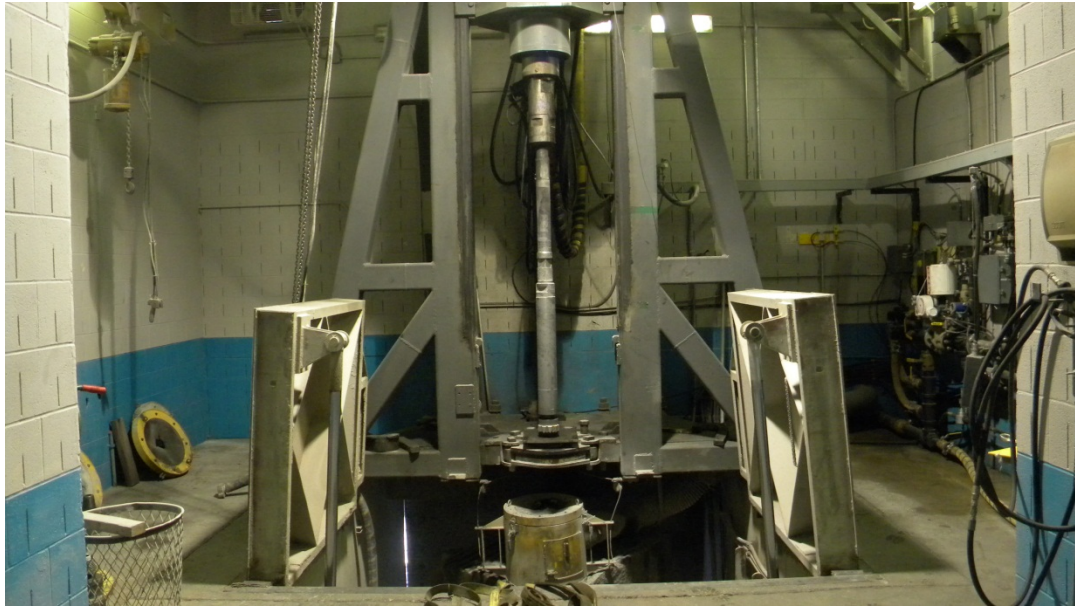
Figure 11. Drill Tower, Showing Basement Access for Rock Sample
