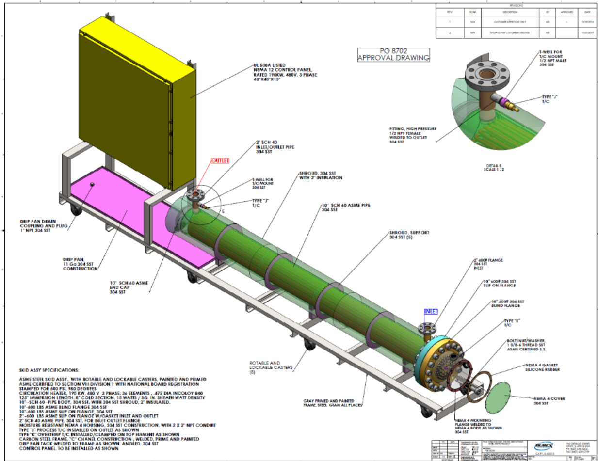
Figure 65. Process gas heater layout
