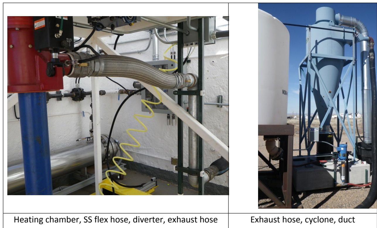
Figure 61. Cyclone discharge subsystem
