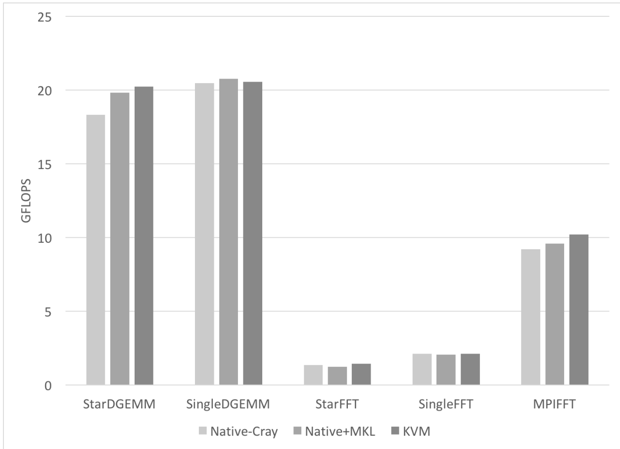
Figure 4.1. Intra-node FLOPS performance
