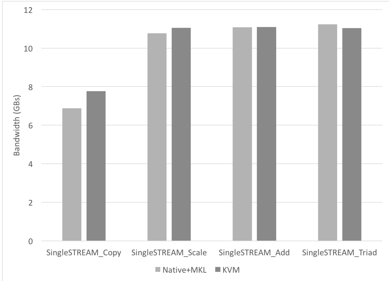
Figure 4.3. Intra-node STREAM performance
