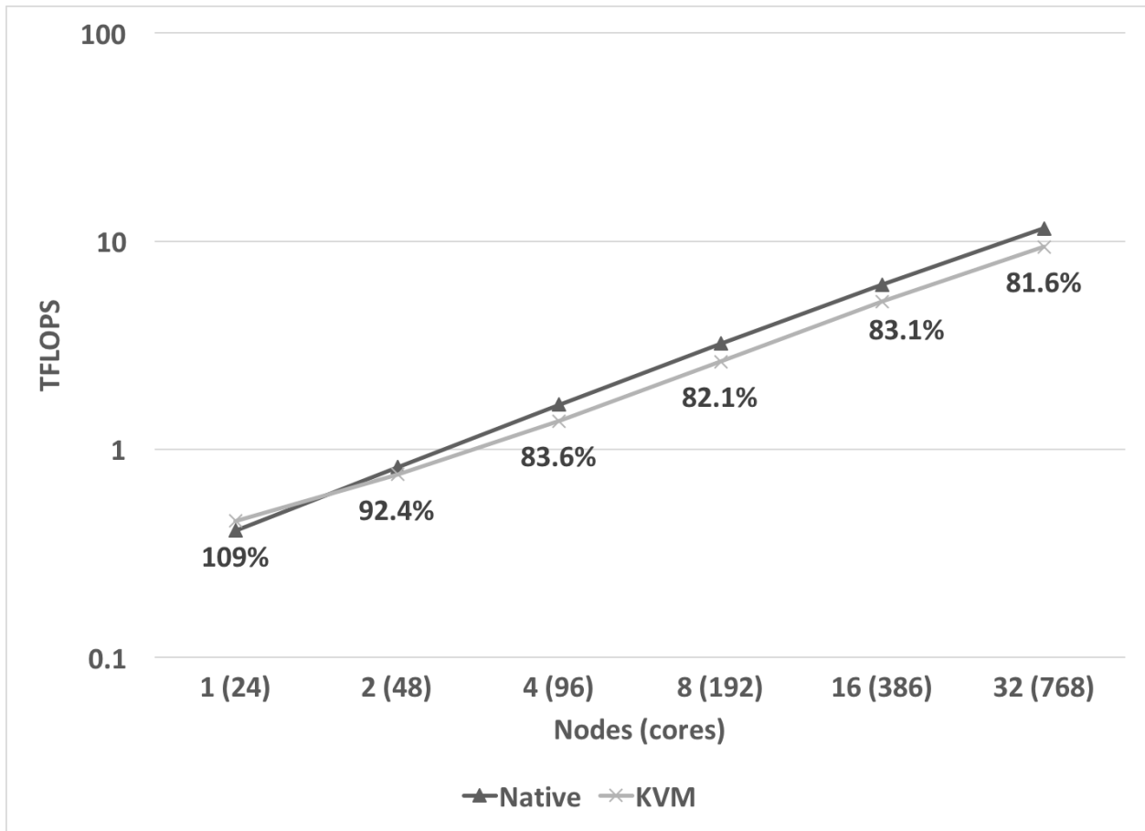
Figure 4.5. Weak Scaling of the High Performance Linpack benchmark to 32 nodes
