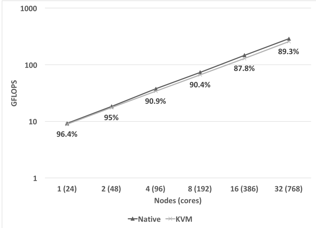
Figure 4.6. Weak scaling of the HPCG benchmark up to 32 nodes
