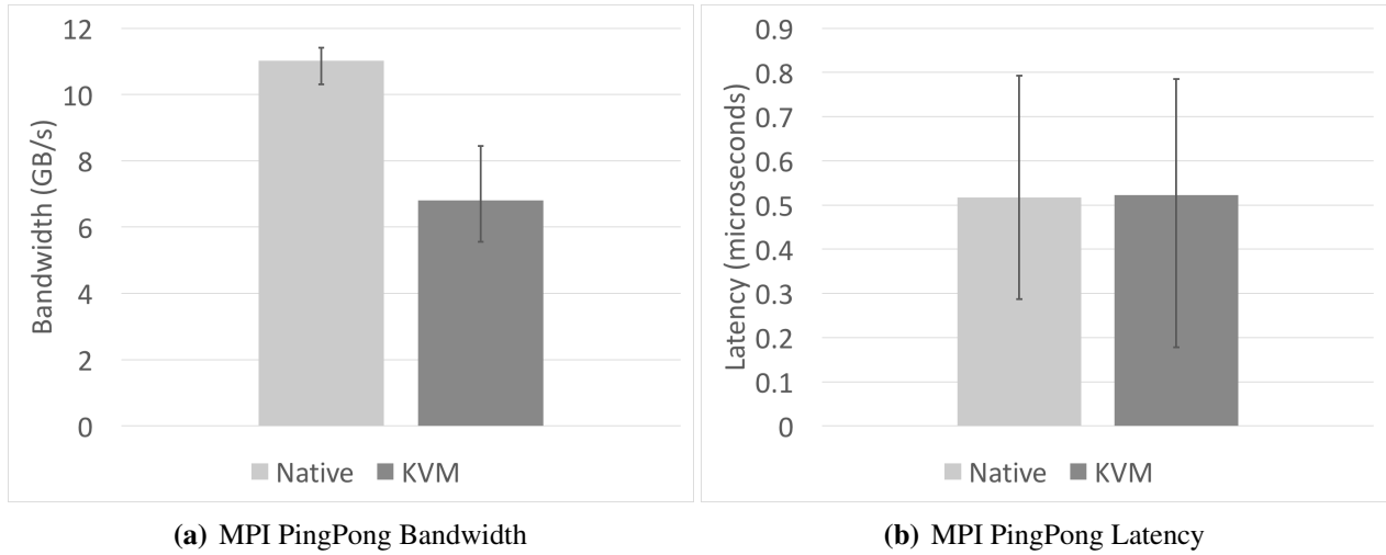
Figure 4.4. HPC MPI intra-node communication performance, with 2MB messages for bandwidth and 8 byte messages for latency
