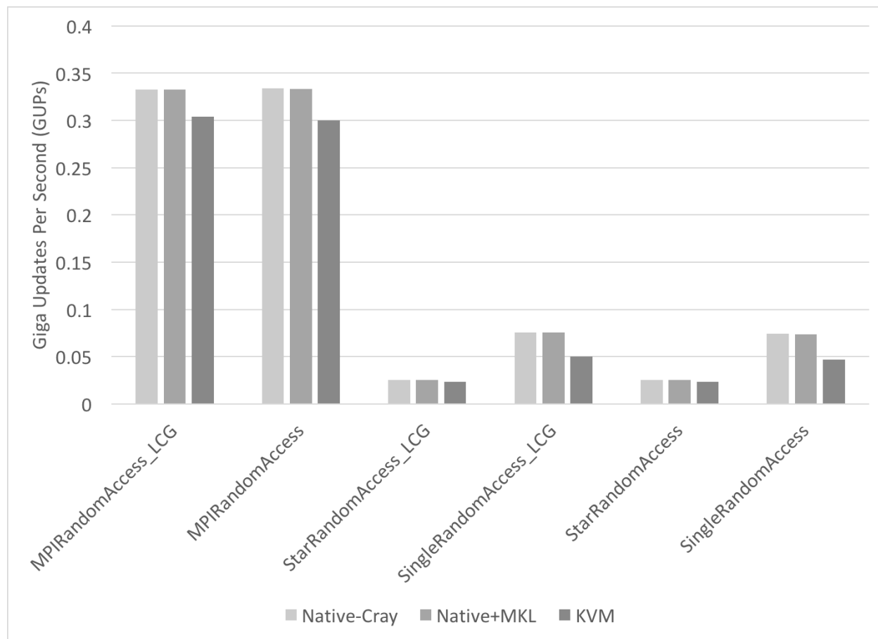
Figure 4.2. Intra-node GUPS performance
