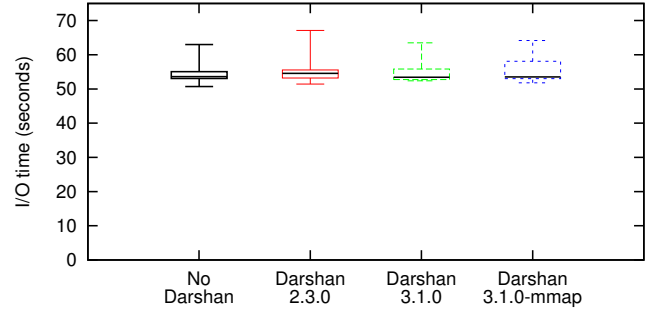
Fig. 2. I/O time reported by an IOR file per-process experiment with and without Darshan instrumentation.
