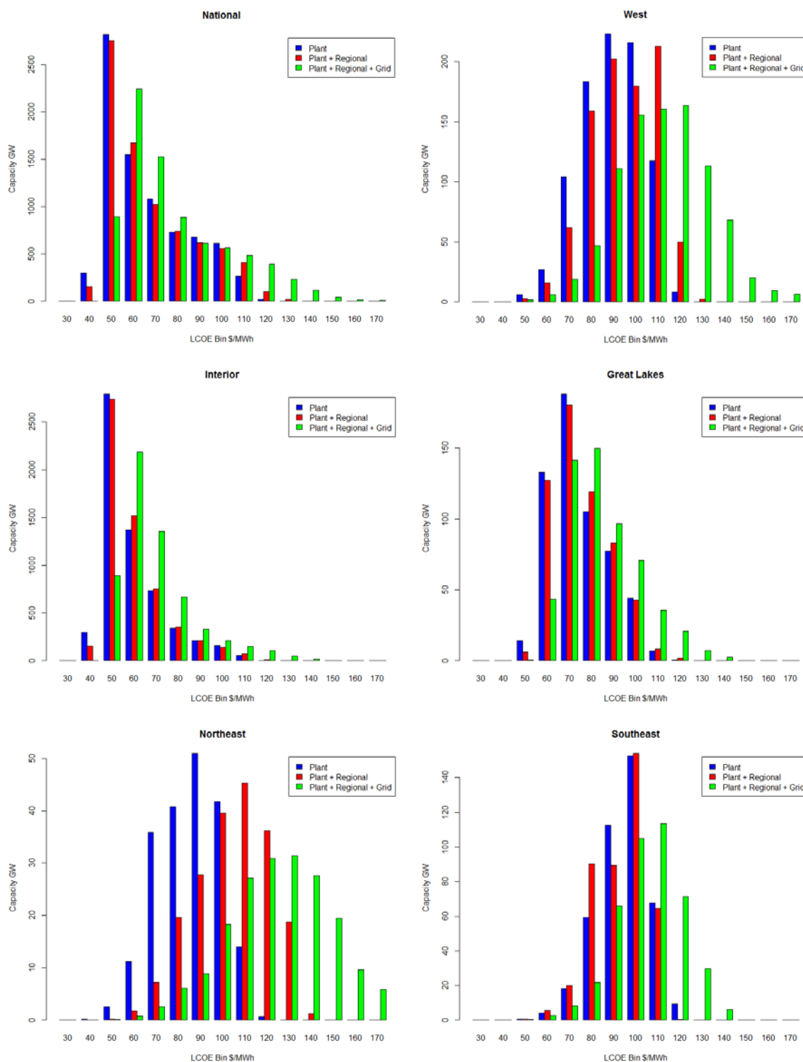
Figure 13. Histogram of wind plant potential capacity for LCOE ranging from $39/MWh to $180/MWh (graphics truncated for visualization). Note that the LCOE bin labels include the lower bound of the histogram bin, and the y-axis varies in each histogram.
