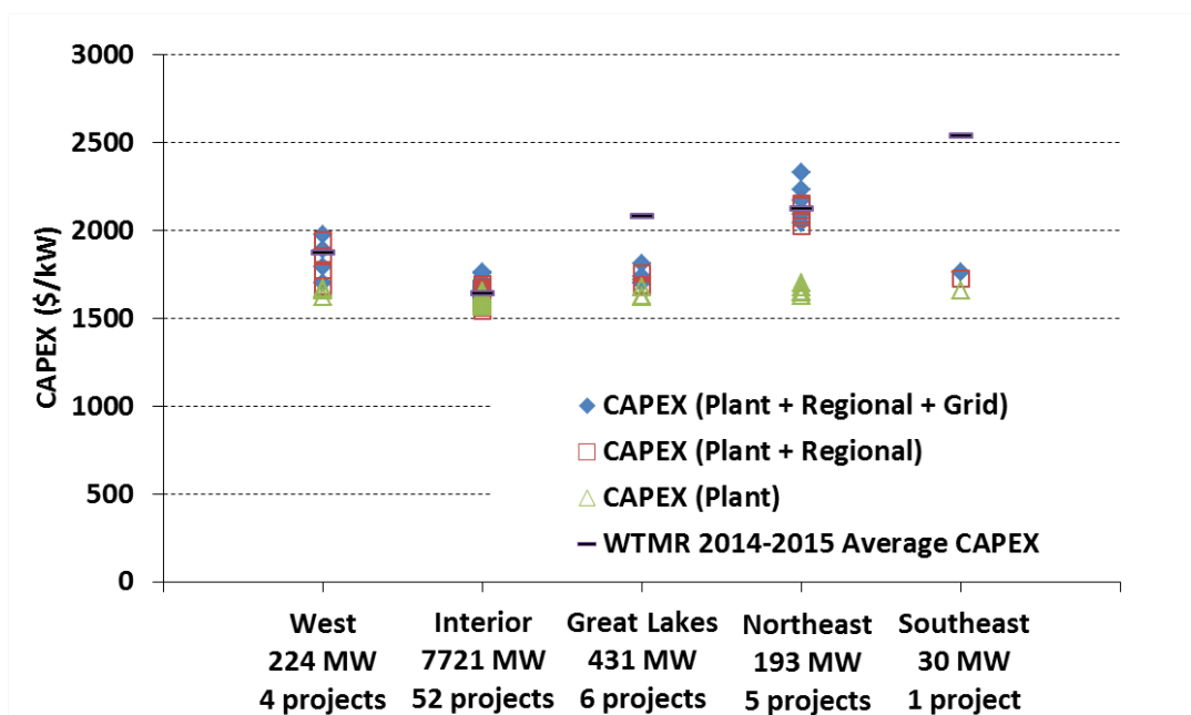
Figure 10. CapEx estimated for locations where projects were installed in 2015 including the wind plant, regional cost increment, and grid connection cost increment (wind technologies market report [WTMR])
