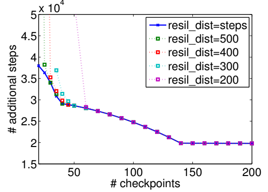
Figure 3: Additional time steps needed for adjointing 10,000 steps
