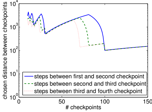
Figure 4: Distance of the first four checkpoints chosen by revolve
