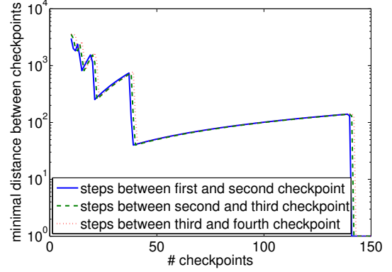
Figure 5: Alternative distance of the first four checkpoints
