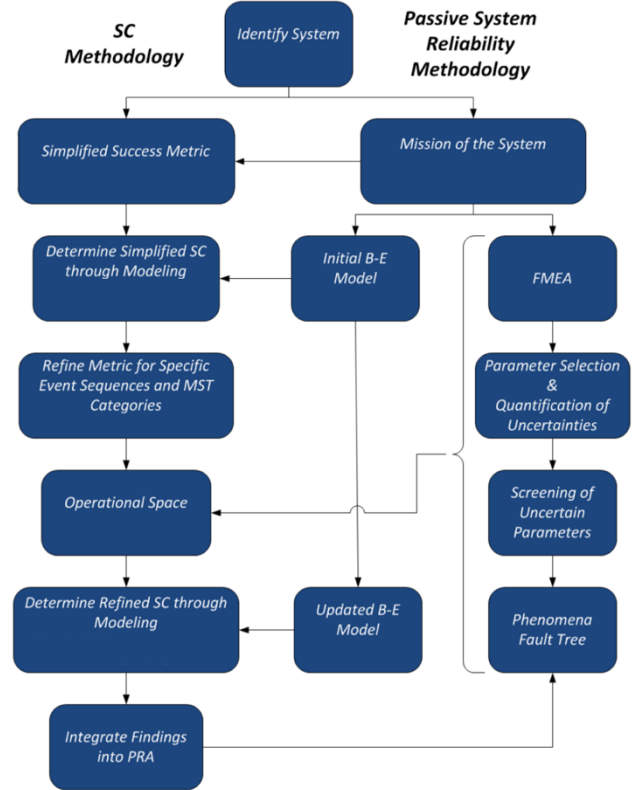
FIG. 1. Passive System Reliability Analysis Procedure
