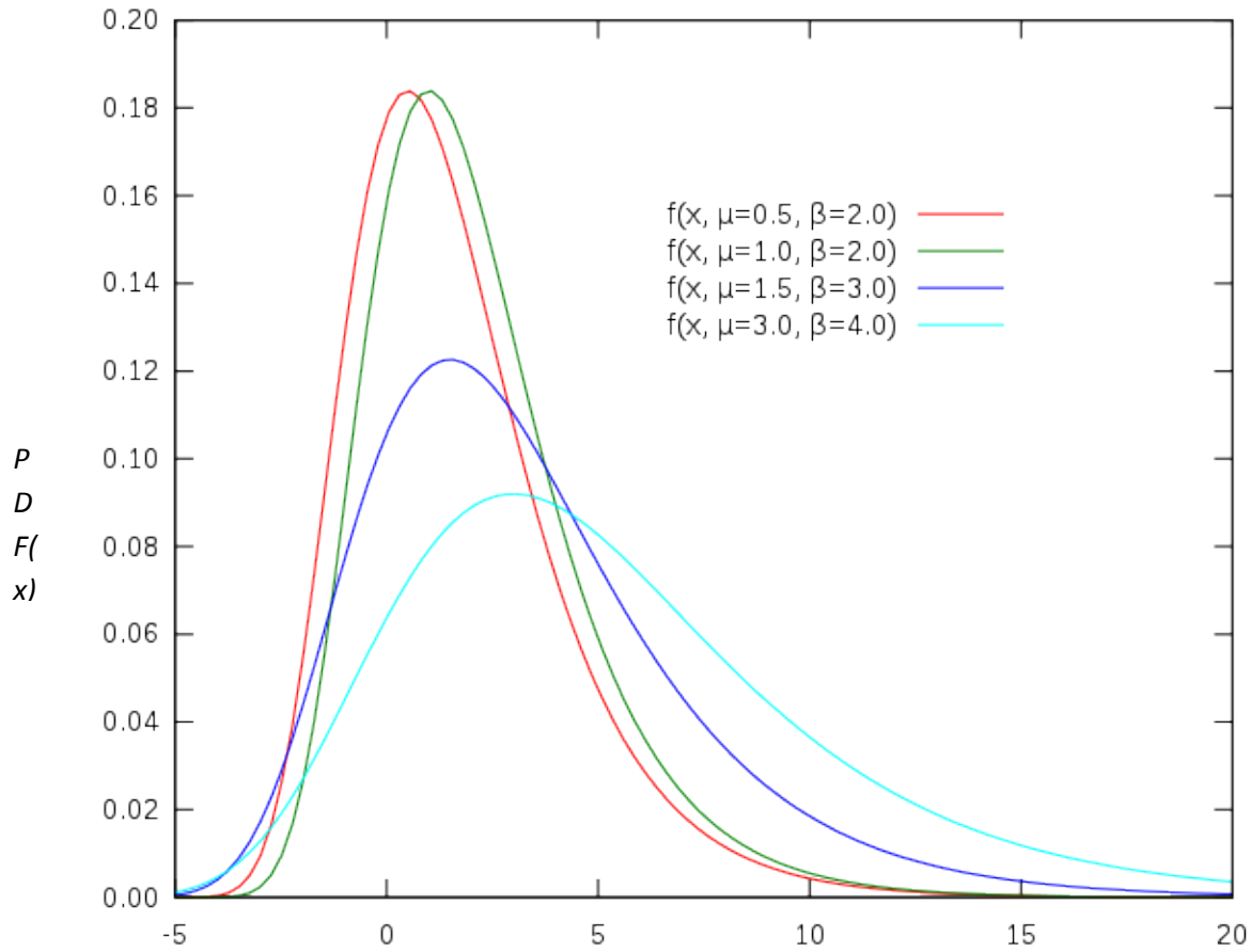
Figure 1: Gumbel Distribution 3
