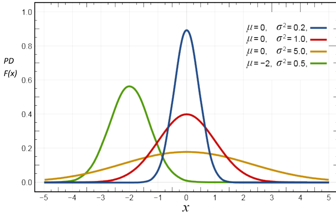
Figure 1: Normal Distribution 3
