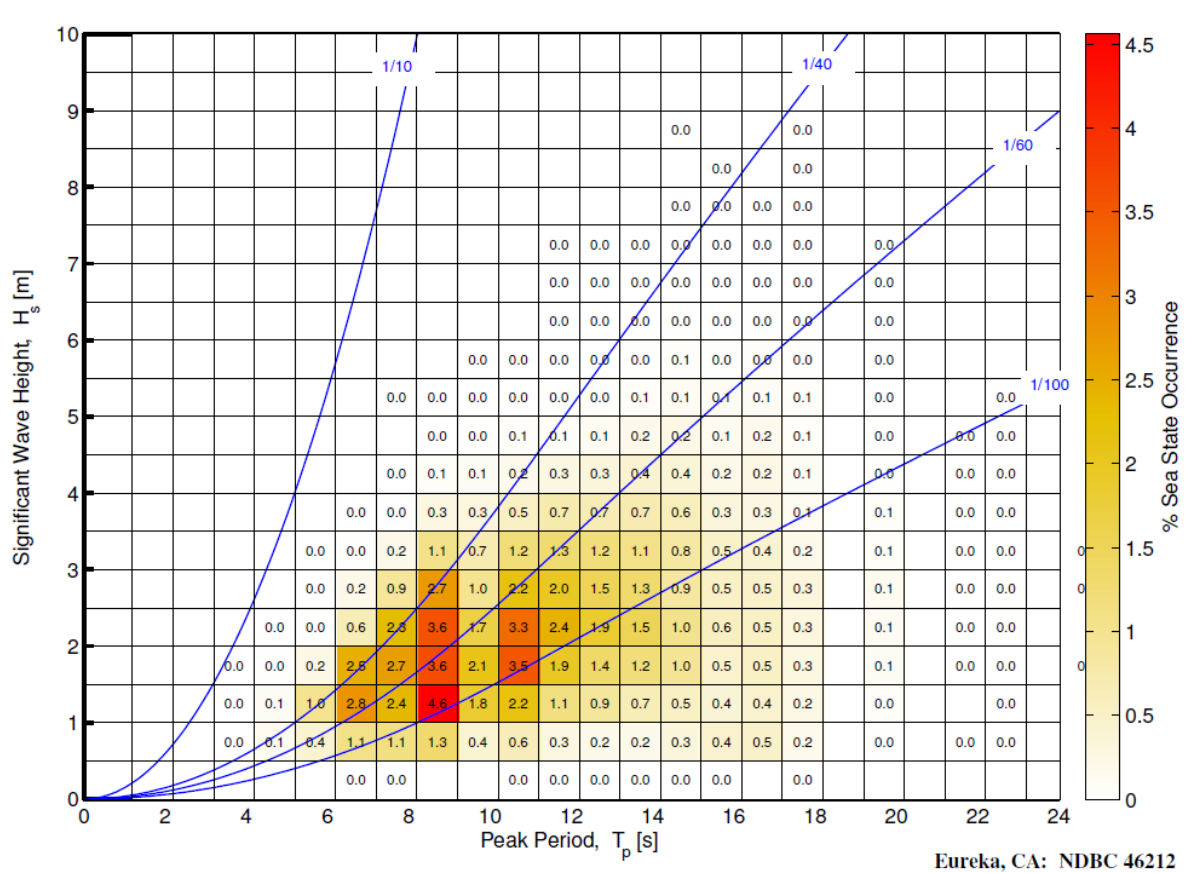
Figure 1. Sea State Occurrence in % per year per bin.
