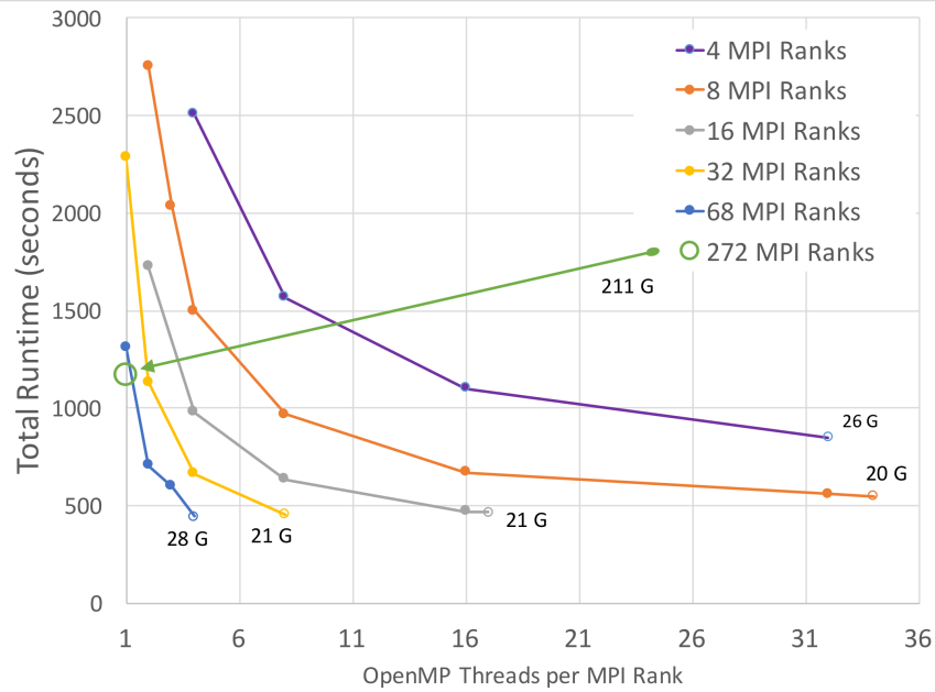
Figure 1: Scaling of Threads on KNL chipset
