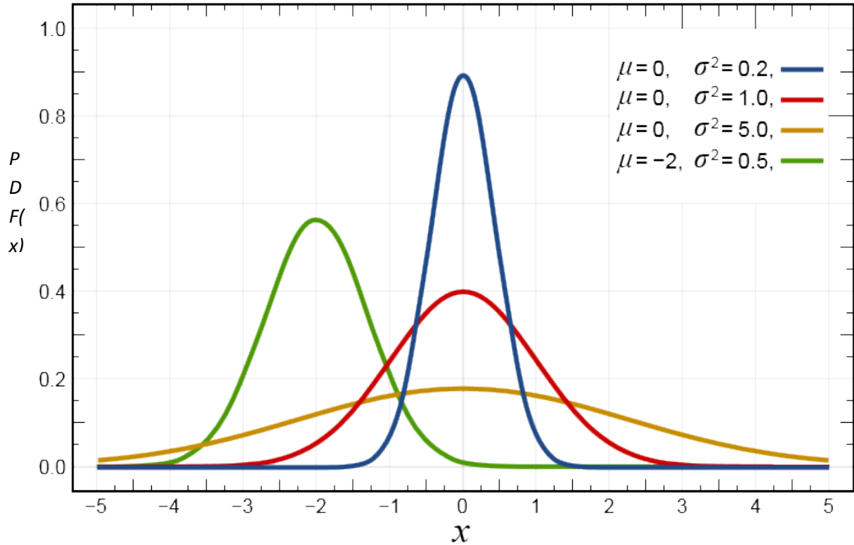
Figure 1: Normal Distribution 3
