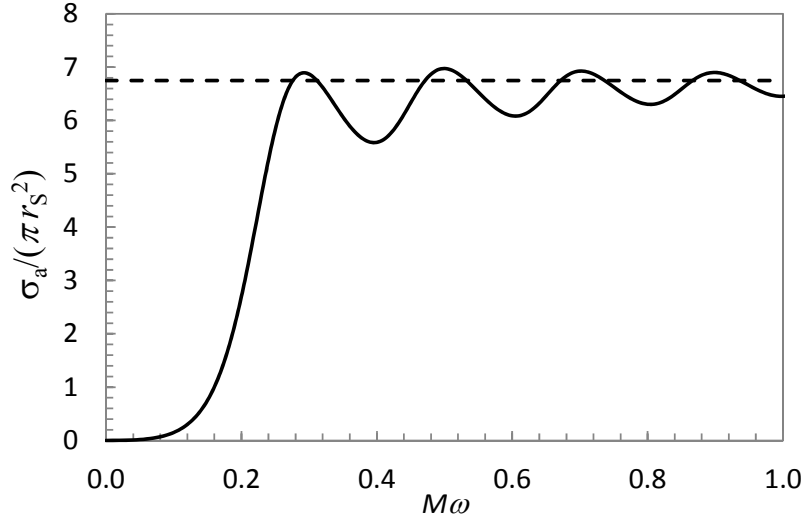
Fig. V.B.1. The black hole photon-absorption cross section as a function of M\omega .
