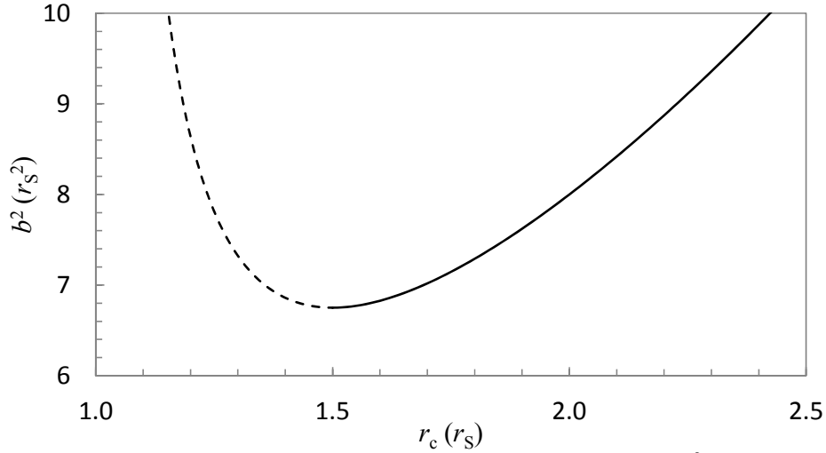
Fig. V.A.2. The relationship between the square of the impact parameter b^2 of a photon incident on a Schwarzschild black hole on the distance of closest approach r_c . The turning point is at r_c = 3/2 and b^2 = 27/4 , and marks the transition between non-capture and capture paths. The solid curve shows the physical solutions with a positive slope. The dashed curve shows the unphysical solutions.
