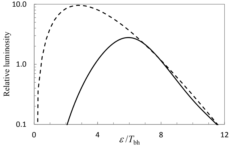
Fig. V.B.2. Luminosity of a black hole calculated using the absorption cross sections displayed in Fig. V.B.1 (solid curve) relative to that obtained using geometrical optics (dashed curve).
