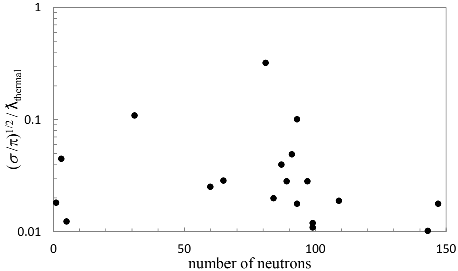
Fig. VII.1. Interaction length scale for thermal-neutron interactions with various nuclei, in units of the reduced wavelength of the corresponding neutrons ( \sim 0.3 Å).
