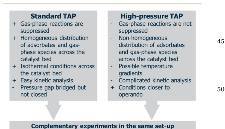
Fig. 4 Advantages, disadvantages and comparison of standard and high-pressure TAP.
