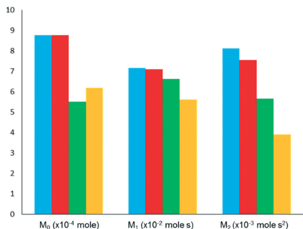
Fig. 14 Comparison of moments ( M_n ) of pulse responses for AMU 40 (argon) at 623 K over Co-Cr-Sn-WOx/ \alpha -Al 2 O 3 for experimental (blue), expanded (red), forced baseline (green) and terminal baseline (yellow).
