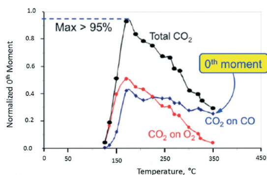
Fig. 10 CO 2 production observed from vacuum pump-probe experiment over a single Pt particle. The black line represents the total CO 2 yield. The red and blue lines represent the CO 2 yield on the oxygen pulse and CO pulse, respectively. 18
