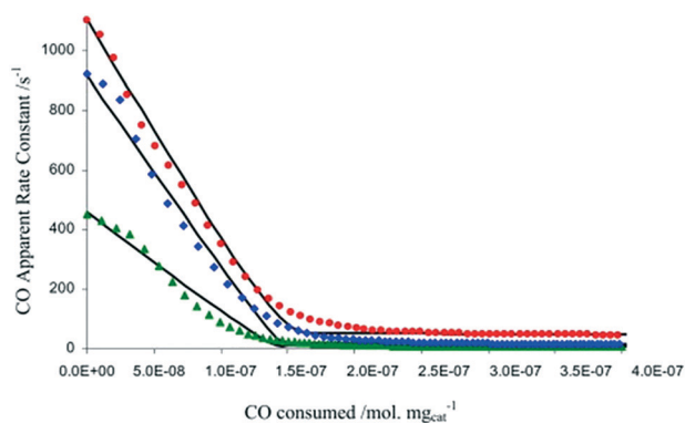
Fig. 7 CO apparent rate coefficient observed in CO multi-pulse experiments at 250 (green), 300 (blue), and 350 °C (red) over 3 mg of 2% Pt/CeO 2 catalyst as a function of the CO consumed. 38
