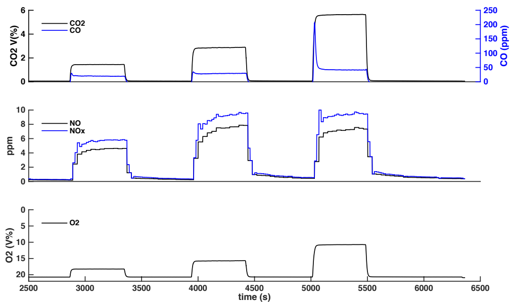
Figure C2: Measured analyte concentrations for on-demand water heater ECOH200DVLN (Trial 1)
