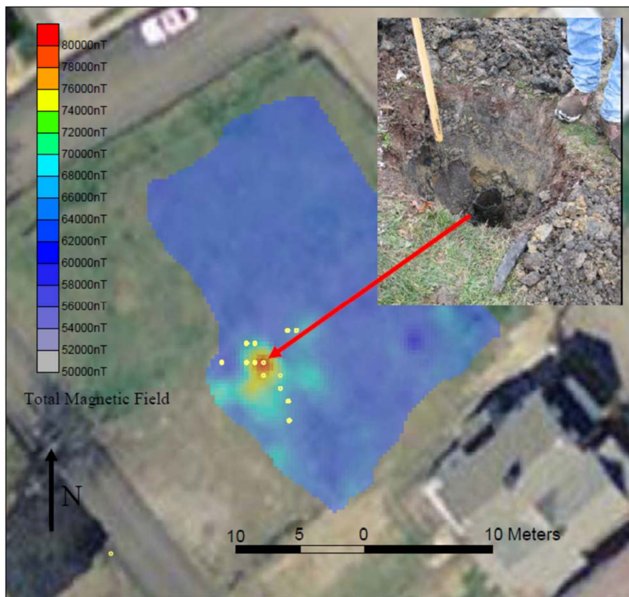
Figure 8: Color-scale magnetic map containing a strong monopole anomaly that denotes the location of an abandoned gas well. Yellow circles indicate locations where CH 4 levels exceeded 100 ppm. Inset is a picture of the gas well casing excavated at this location.
