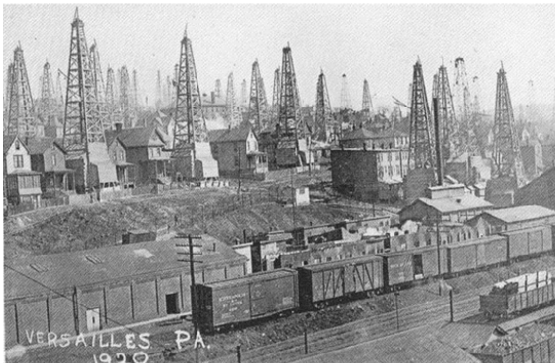
Figure 2: Photograph of Versailles Borough, Pennsylvania in 1920 showing gas well derricks interspersed between houses (photo courtesy of McKeesport Regional History and Heritage Center http://mckeesportheritage.org/research ).
