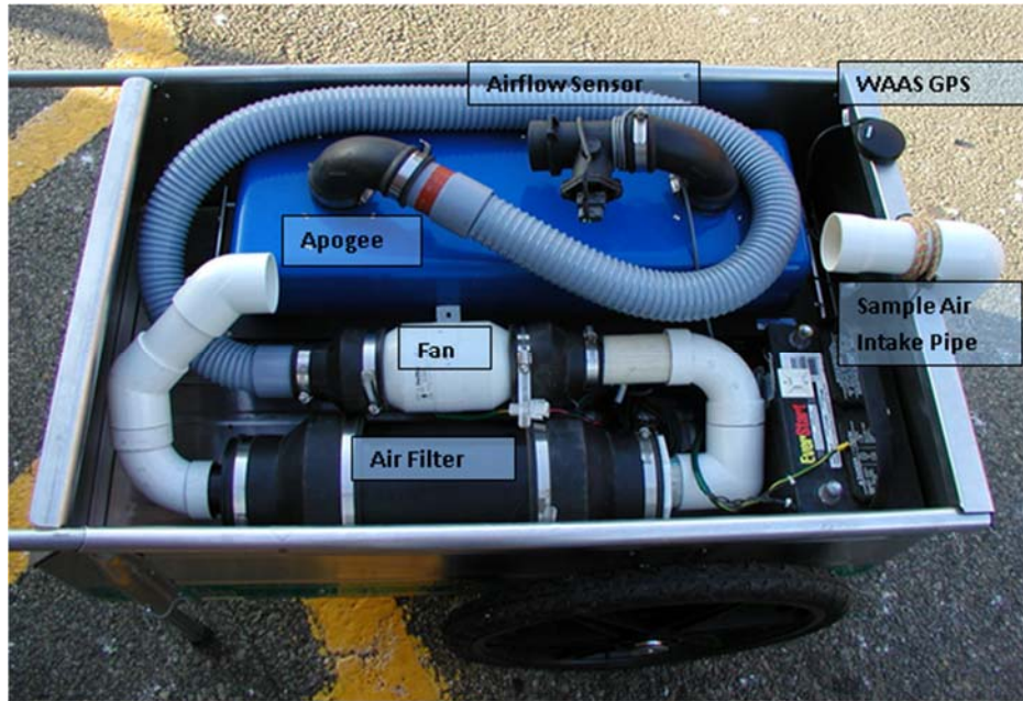
Figure 5: An LDS was deployed in a lightweight cart to detect trace amounts of CH 4 emanating from leaking wells and other sources. The tablet computer and a portion of the inlet pipe were removed for clarity.
