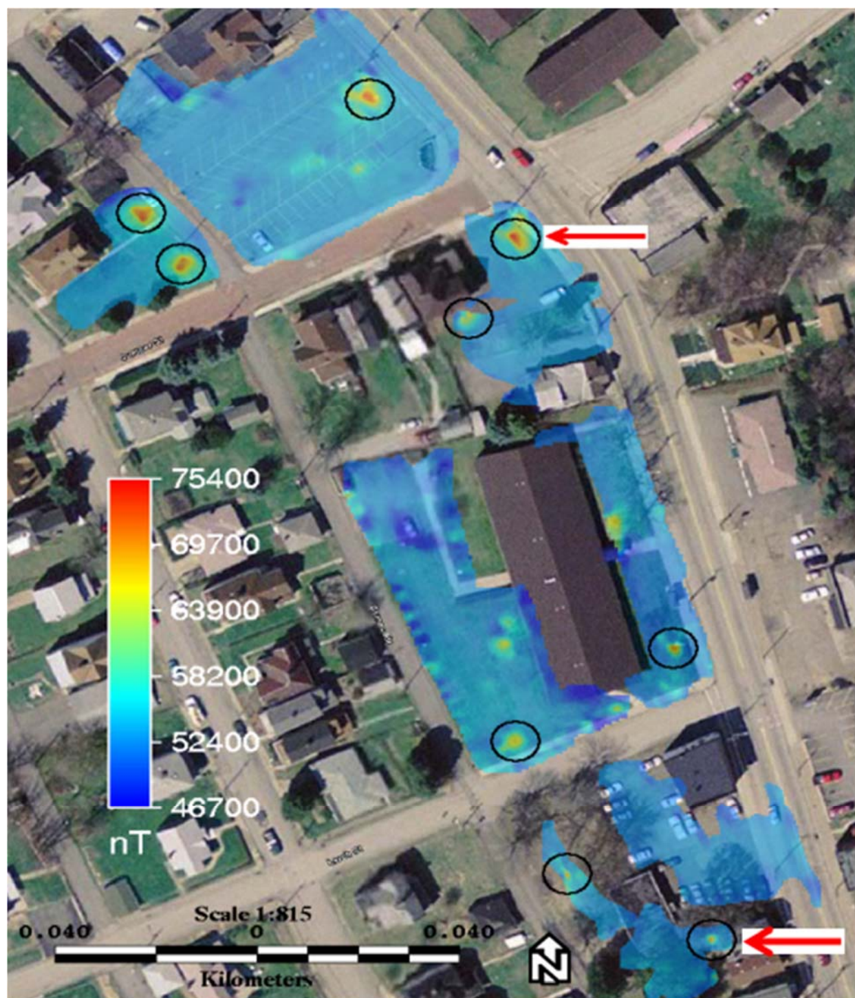
Figure 12: Color-scale map of total field magnetic data overlain on georeferenced Google Earth™ imagery from Versailles Borough. Circled features are magnetic anomalies exceeding 60,000 nT and believed to be unmarked wells. Red arrows denote the locations of well-type magnetic anomalies that are associated with CH 4 anomalies.
