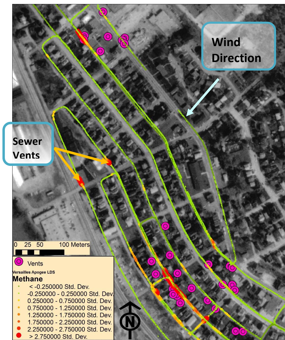
Figure 7: Map showing areas of above-normal CH 4 concentrations detected by a truck-mounted CH 4 survey of Versailles Borough. Methane concentrations are represented by symbols with graduated size and color; magenta symbols denote the locations of CH 4 mitigation vents.
