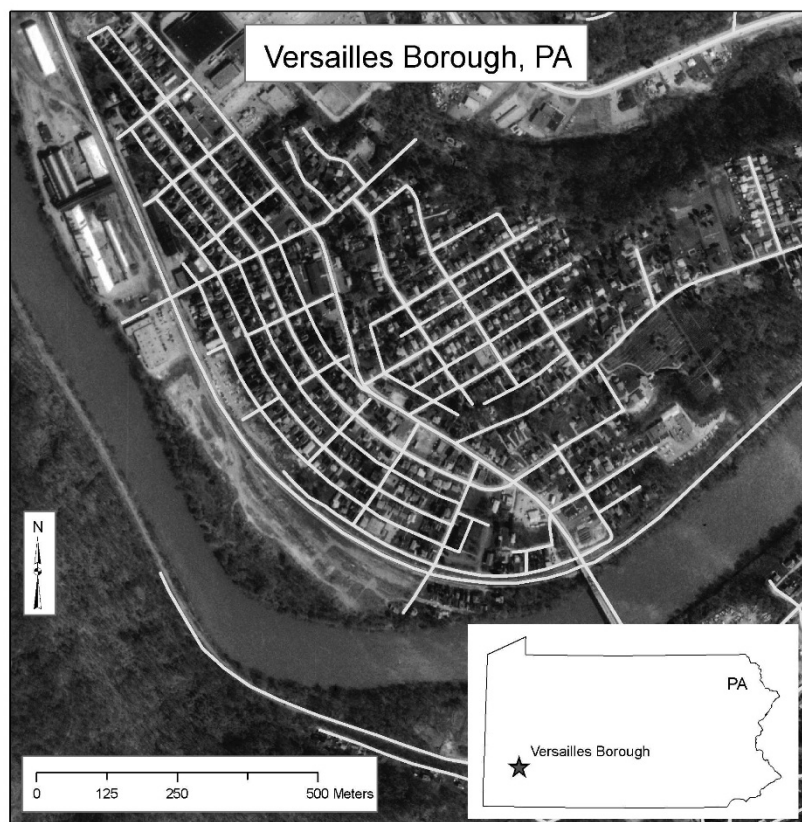
Figure 1: Location map of Versailles Borough, PA.
