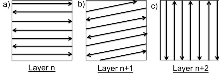
Figure 1: Raster scan strategy utilized as default by the electron beam heat source depicting an exaggerated rotation of the scan pattern within the build plane for a) Layer n b) Layer n+1 c) Layer n+2.
