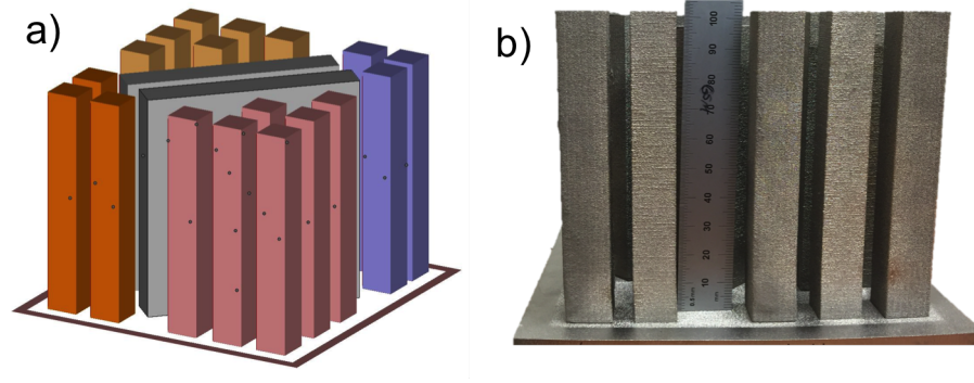
Figure 3: Build layout used for the fabrication of mechanical test specimen blanks in this study a) CAD Model b) Front view of completed EBM build.
