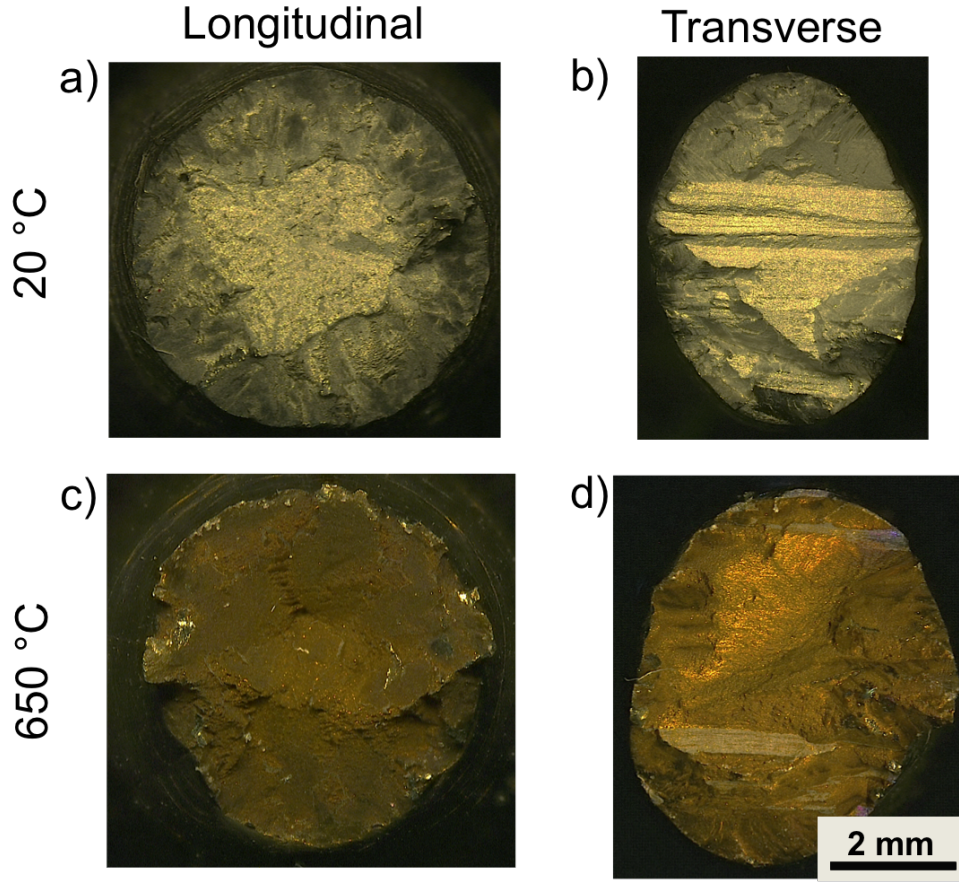
Figure 9: Optical micrographs of the tensile fracture surfaces of the columnar grained material fabricated using the standard raster fill within the a) Longitudinal orientation at 20 °C b) Transverse orientation at 20 °C c) Longitudinal orientation at 650 °C d) Transverse orientation at 650 °C.
