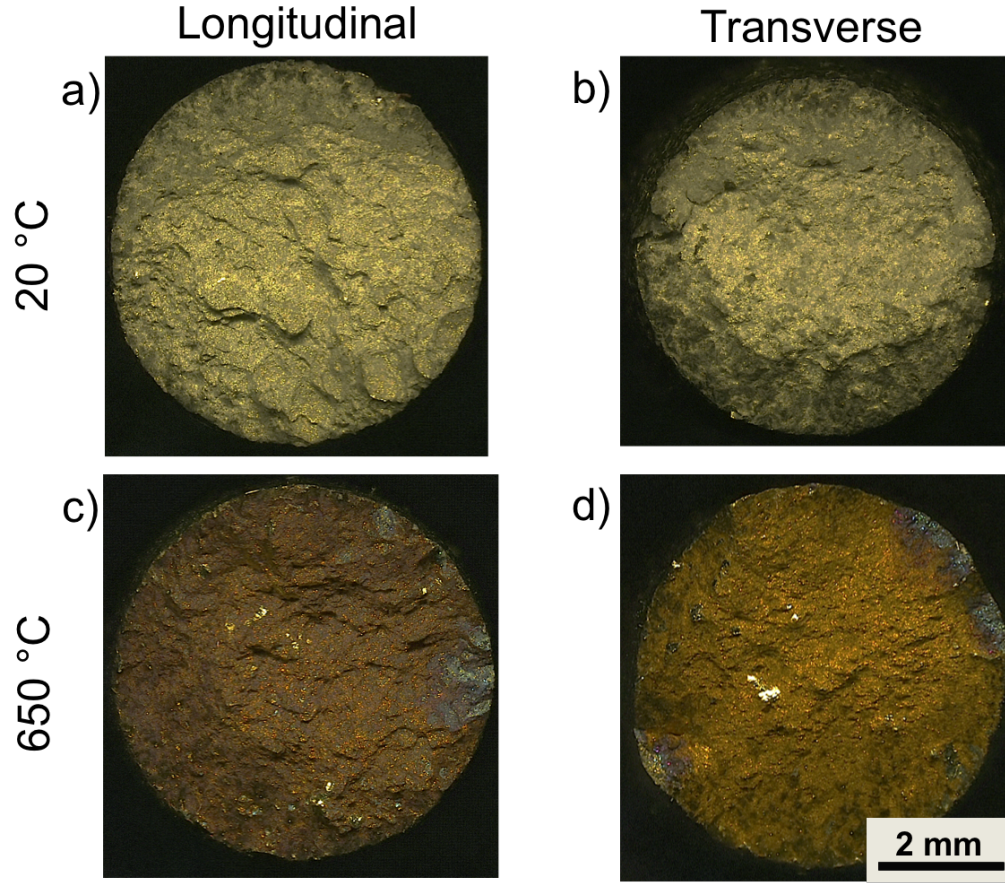
Figure 10: Optical micrographs of the tensile fracture surfaces of the equiaxed grained material fabricated using the point heat source fill within the a) Longitudinal orientation at 20 °C b) Transverse orientation at 20 °C c) Longitudinal orientation at 650 °C d) Transverse orientation at 650 °C.
