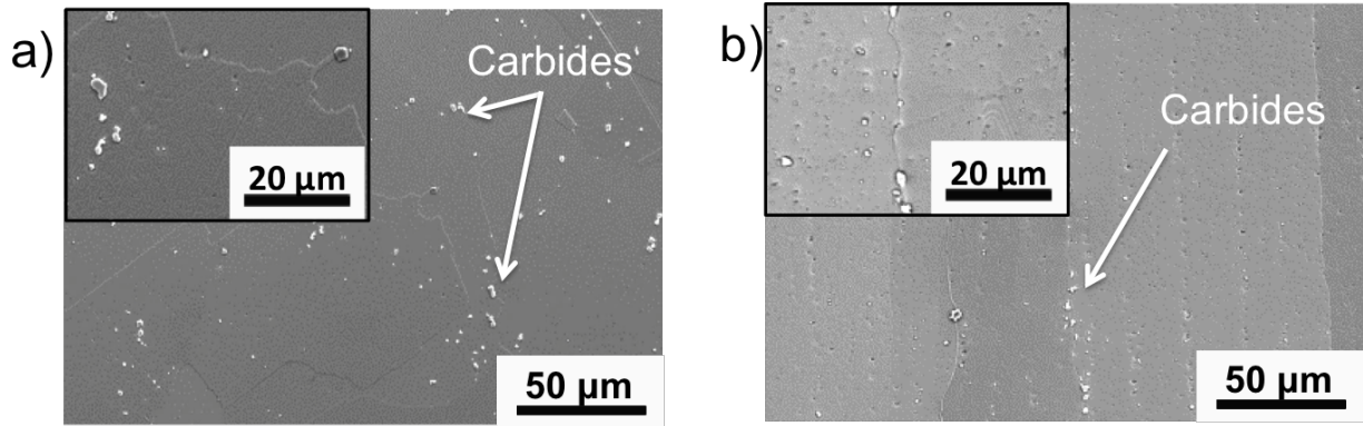
Figure 7: Representative secondary electron SEM images depicting the location of carbides within the a) Equiaxed grained material fabricated with the point heat source fill b) Columnar grained material fabricated with the raster scan strategy.
