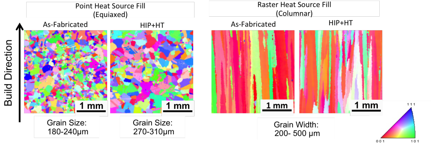
Figure 6: EBSD grain orientation maps before and after post-processing for a) Material fabricated through the point heat source fill indicating a random texture b) Columnar grained material fabricated through the standard raster scan strategy.
