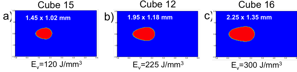
Figure 5: Simulated melt pool shapes and sizes for 10 neighboring spots for a) Cube 15 b) Cube 12 c) Cube 16.
