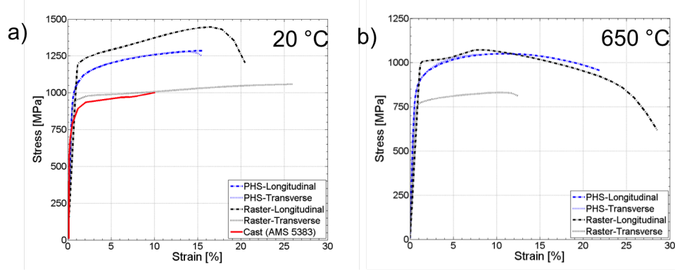
Figure 8: Stress-strain response of EBM Inconel 718 fabricated using raster scan strategy (Raster) and point heat source fill (PHS) at a) Room temperature in relation to cast and wrought Inconel 718 b) 650 °C.
