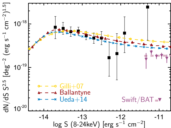
FIG. 5.— The NuSTAR 8 – 24 keV number counts compared to Swift / BAT (bold dashed line) (Ajello et al. 2012). The hatched region indicates the uncertainty in the overall fit from Ajello et al. (2012). We convert the BAT 15–55 keV band to the 8 – 24 keV band using a power law with photon index \Gamma = 1.7 (the best-fit to the average BAT AGN spectrum in the 15 – 55 keV band). The dashed line with triangles shows predictions from the CXB synthesis model of Ballantyne 2011 updated to use the Ueda 2014 luminosity function. The dashed line with crosses shows the population synthesis model from Ueda et al. (2014). The dashed line with circles shows predictions from the CXB model from Gilli, Comastri & Hasinger (2007). The plotted errors are 1- \sigma .
