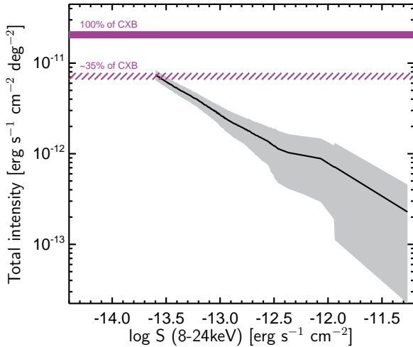
FIG. 6.— Total intensity as a function of 8 - 24 keV flux of the resolved sources in the sample included in this work. The horizontal lines indicate 35% (hatched line) and 100% (solid line) of the cosmic X-ray background (CXB). The width of the lines indicates the range of normalizations determined by different instruments (see Table 1 for references). At the faint end of the surveys included here NuSTAR is resolving \sim 35\% of the CXB.
