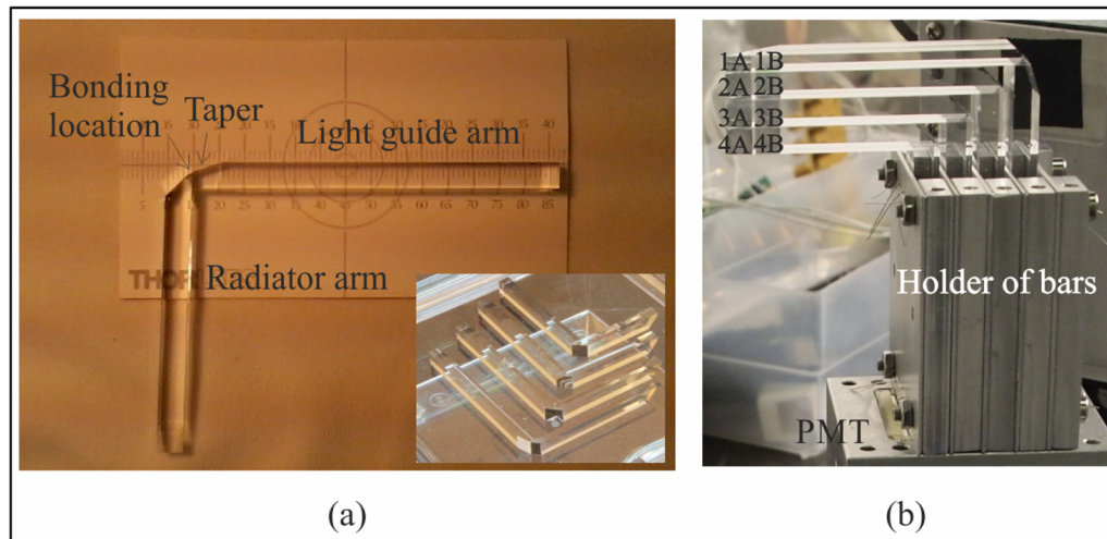
Fig. 2. (a) Example of a fused silica bar with the taper and a set of bars, (b) the set of 2x4 bars forming the ToF prototype.
