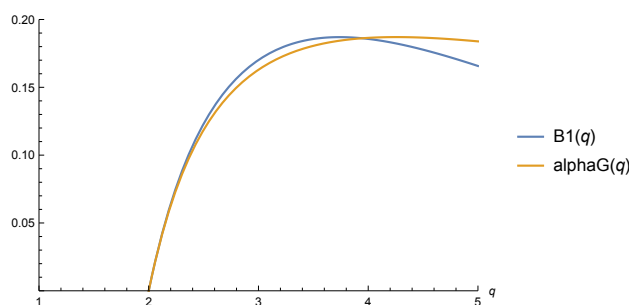
Figure 1. The red line represents \alpha_G and the blue line represents the right hand side of eq. (2.40).
