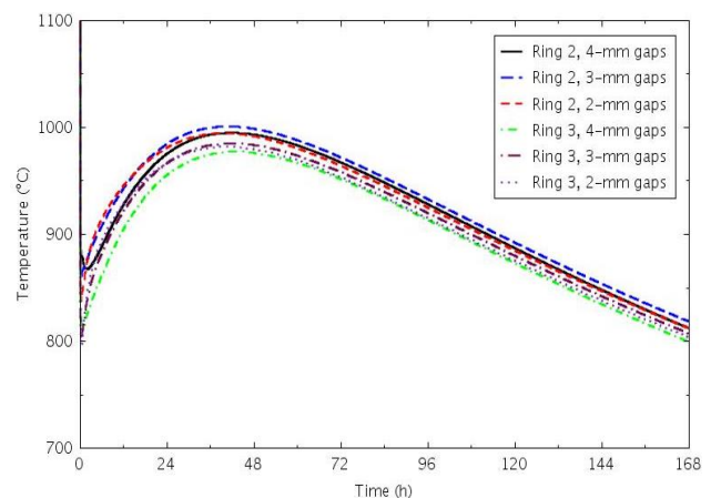
Fig.10. Peak fuel temperatures for a PCC transient.
