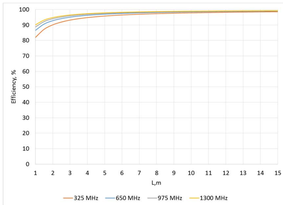
Figure 2-7 Efficiency versus the linac length for different frequencies for 10 MeV, 10 MW linac. The efficiency is not an issue, but power losses on the cavity wall may be critical.
