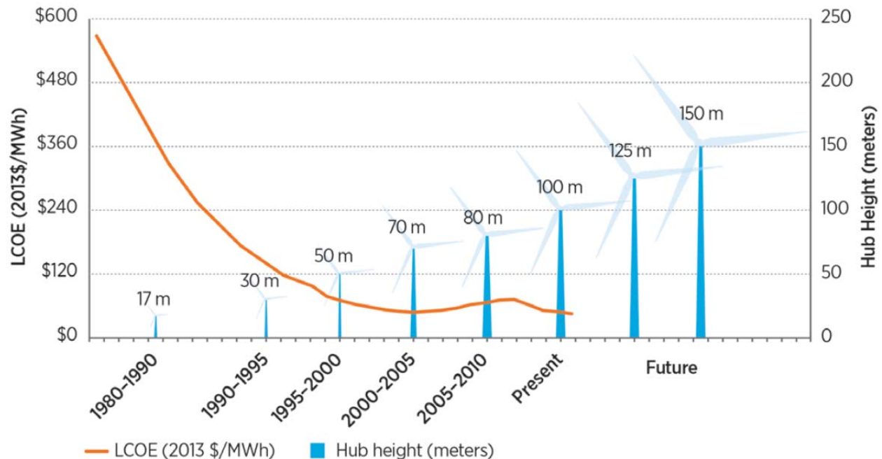
Figure 3-1 Wind technology scale up trends and LCOE [3-7].
