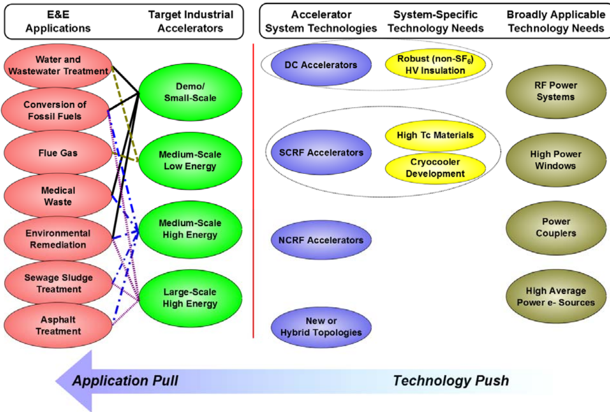
Figure 2-3 Accelerator applications in E&E require capabilities beyond today's state of the art. Candidate technologies require R&D to fill capability gaps; much of the R&D is broadly applicable across potential technologies.
