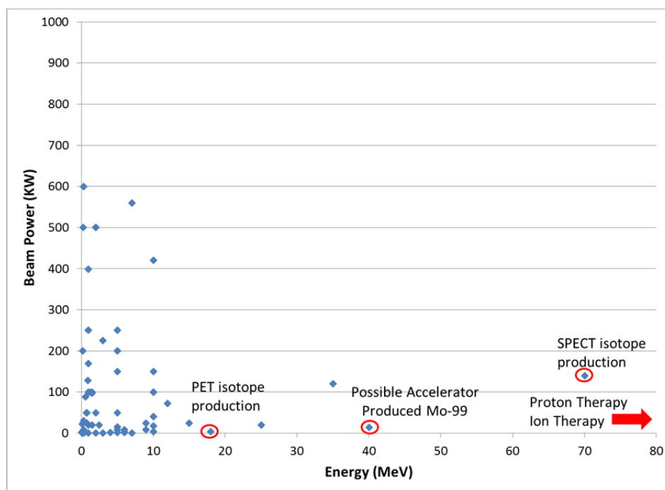
Figure 2-5 Survey of beam energy and beam power of industrial accelerators in use at present. Well known medical applications of accelerators shown as reference.
