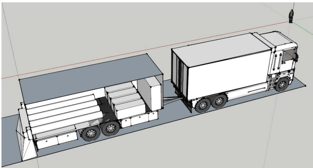
Figure 2-2 Illustration of a mobile, high-power electron accelerator to drive reaction chemistry in roads.
