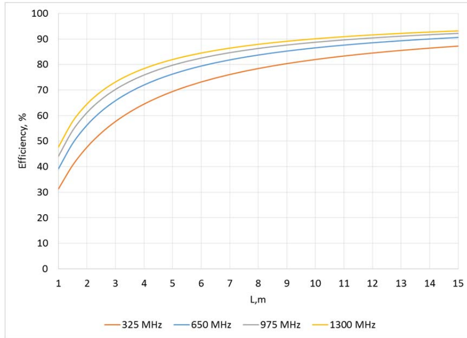
Figure 2-6 Efficiency versus the linac length for different frequencies for 10 MeV, 1 MW linac. Efficiency is ~90% for the ~10-m long linac at 1300 MHz.
