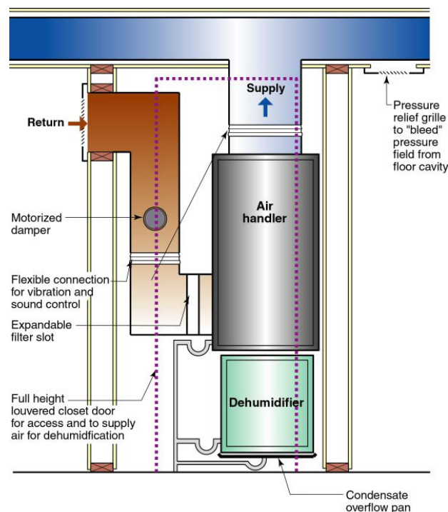
Figure 19. Dehumidifier—In ducted return system
