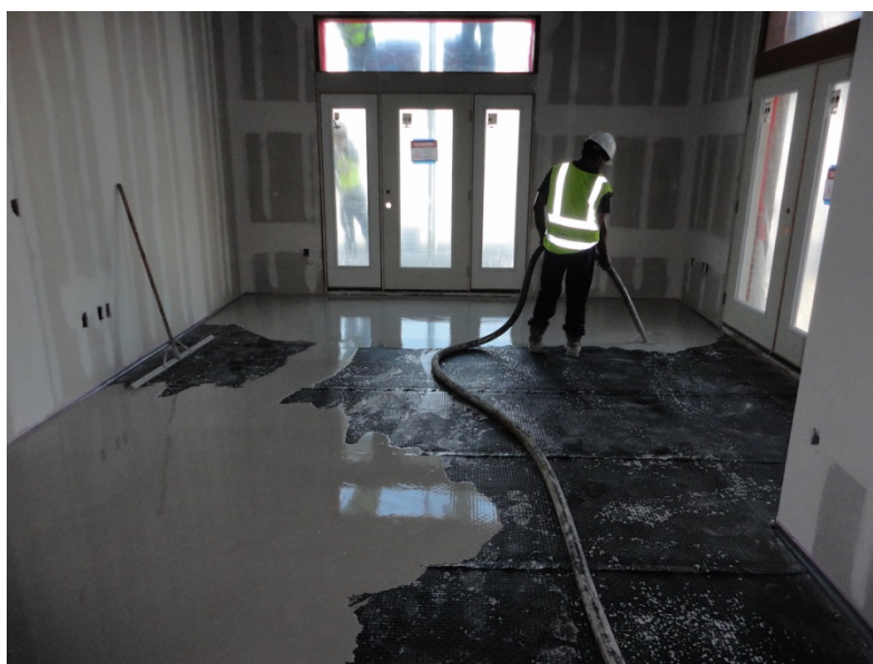
Figure 4. Floor assembly air sealing—Floor assemblies that are soundproofed and fireproofed with liquid gypsum subflooring result in airtight wall assemblies at floor to wall connections
