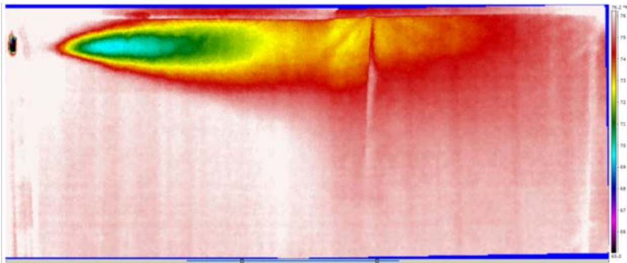
Figure 17. IR photo of the black felt screen during medium-speed cooling system operation (temperature scale in °F)
