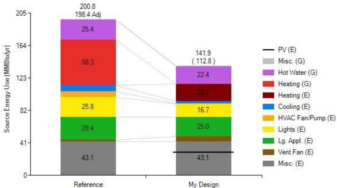
Figure 2. BEopt results
