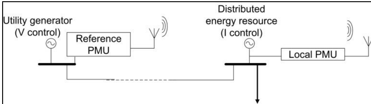
Figure 8. Schematic representation of an implementation of a synchrophasor-based islanding detection method.
