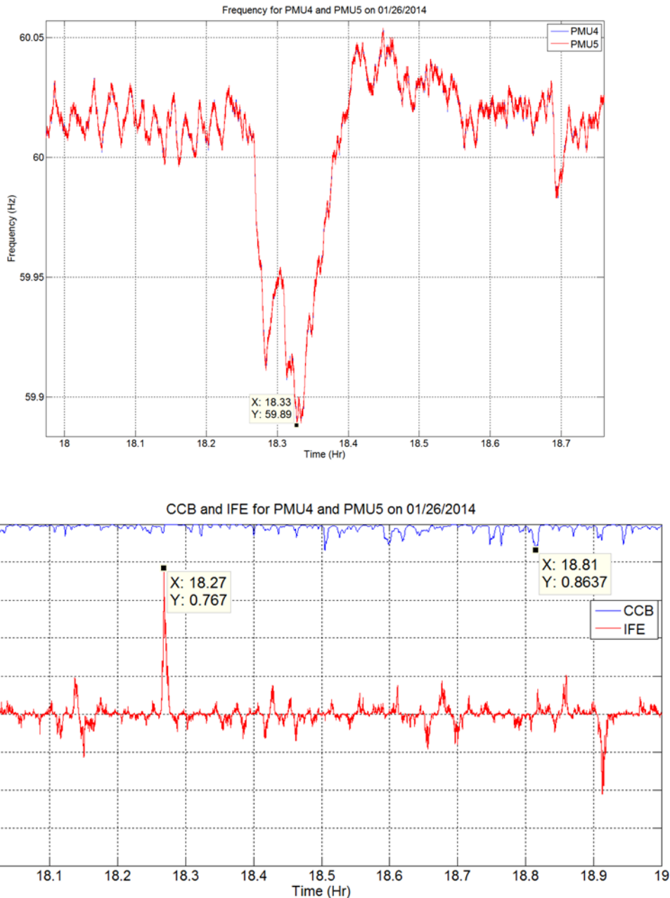
Figure 11. Example of a significant frequency event on the system, triggered by the loss of a large wind farm, and the corresponding CCB + IFE results.
