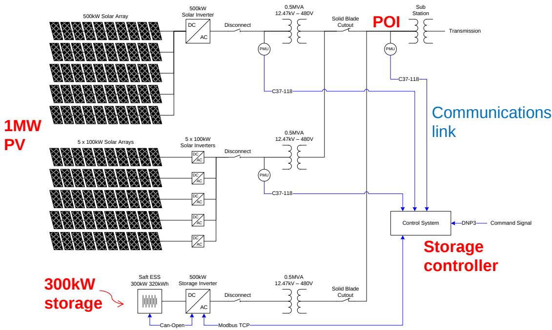
Figure 28: Block diagram for a typical system with ramp controls illustrating POI, PV system, and BIS
