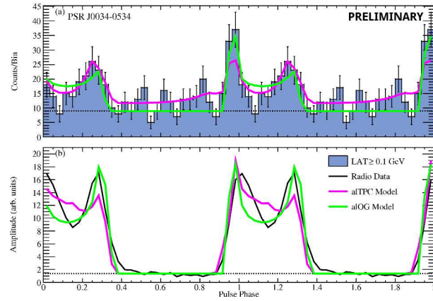
Figure 2: LC fits for PSR J0034–0534 using aLOG / alTPC models. Panel (a) shows the gamma-ray data, while panel (b) shows the radio data.
