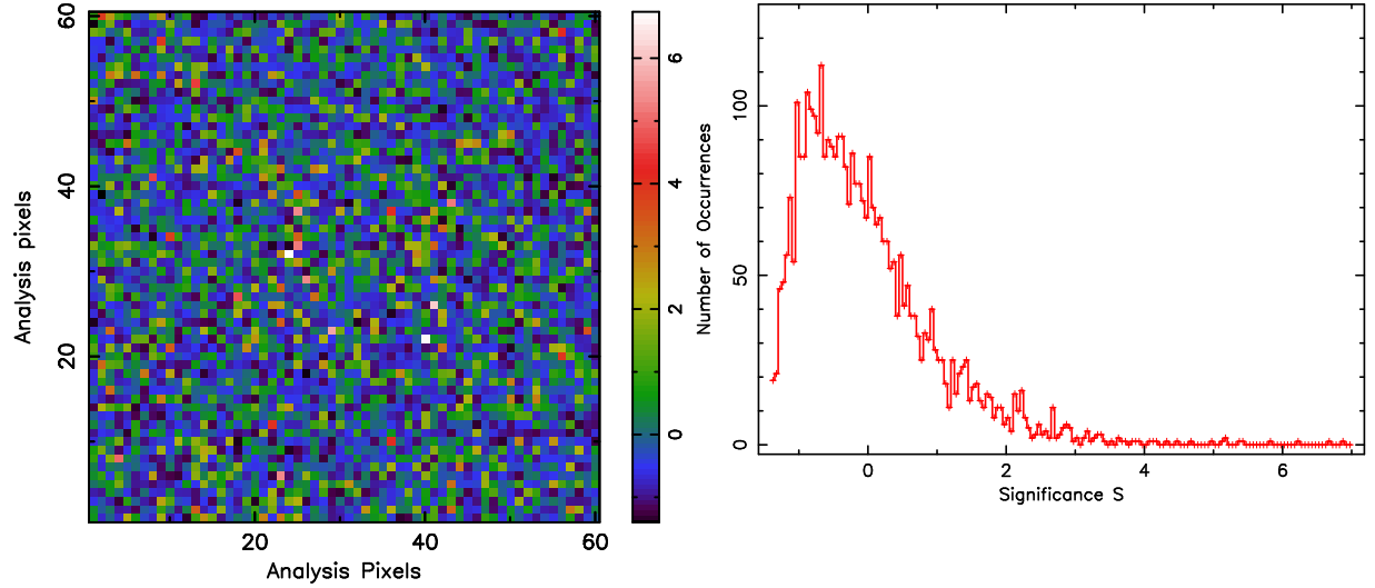
Fig. 4.— Left: Image of the significance measure S_i \equiv (\chi_i^2 - \nu_i)/\sqrt{2\nu_i} of sample counting-rate variations amongst the 5 observations. North is up and the pulsar is at (30,30) in the displayed analysis-pixel coordinates. Right: Histogram of number of occurrences of each value in the image to the left.
