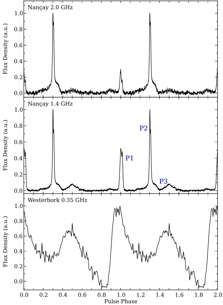
Fig. 1.— Phase-aligned radio light curves of PSR B1821–24, with two pulsar rotations shown for clarity; the peak heights in each panel are normalized independently. From top to bottom: 2 GHz Nançay profile, 1.4 GHz Nançay profile, and 0.35 GHz Westerbork profile. We denote the second-highest radio peak at 1.4 GHz, near phase 0, as P1; the highest radio peak at 1.4 GHz, near phase 0.3, as P2; and the lowest radio peak at 1.4 GHz, near phase 0.5, as P3. Both P1 and P3 are also visible at 0.35 and 2 GHz while P2 has no obvious counterpart at 0.35 GHz.
