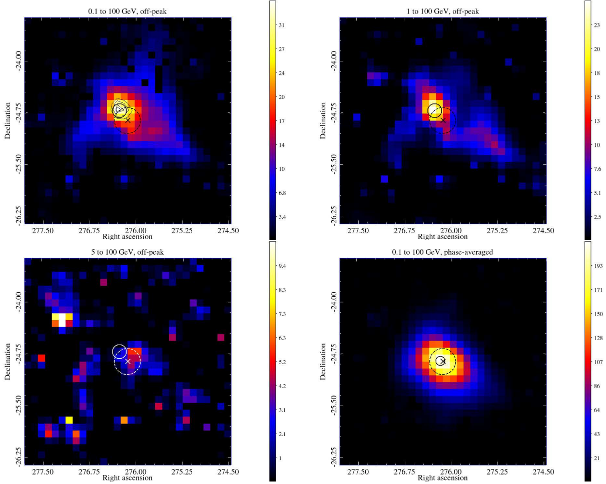
Fig. 3.— TS maps in the off-peak interval of PSR B1821–24 using events from 0.1 to 100 GeV ( top left ), 1 to 100 GeV ( top right ), and 5 to 100 GeV ( bottom left ) and the entire phase interval from 0.1 to 100 GeV ( bottom right ). The TS maps cover 3^\circ \times 3^\circ , centered on the timing position of PSR B1821–24, and have pixels 0.1^\circ on a side. The timing position of PSR B1821–24 is indicated by the X-point, the best-fit LAT position and positional uncertainty from the corresponding phase interval by the solid circle, and the tidal radius of M28 by the dashed circle. The thin black contours in the top left panel represent the 50, 68, 95, and 98% confidence levels.
