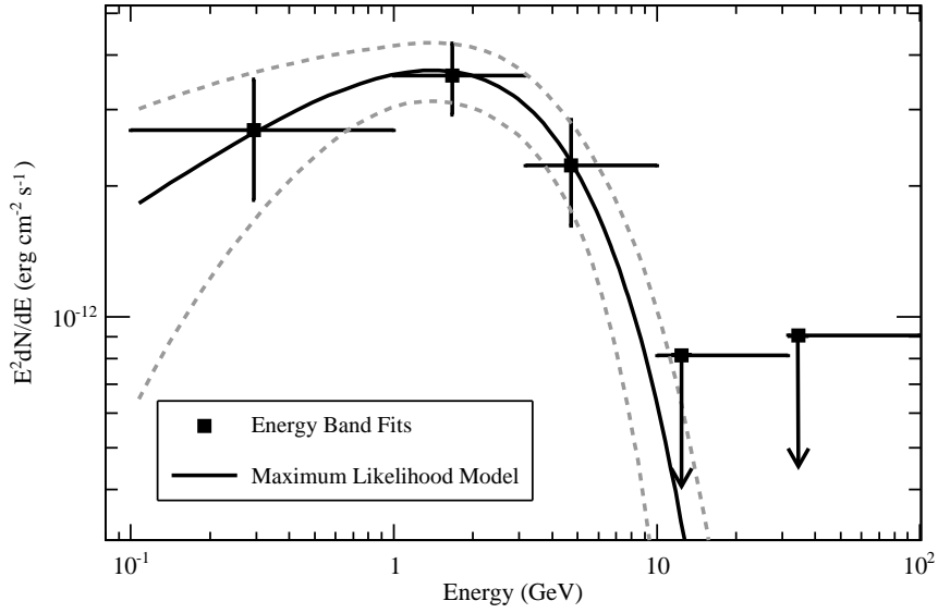
Fig. 4.— Phase-averaged gamma-ray spectrum of PSR B1821–24 with the off-peak source included in the model. The black line shows the best-fit model from the likelihood fit over the full energy range; dashed lines show the 1\sigma confidence region. The pulsar was assumed to have a power-law spectrum in each energy band and required to be found with a TS of at least 9 or else a 95% confidence-level upper limit was calculated.
