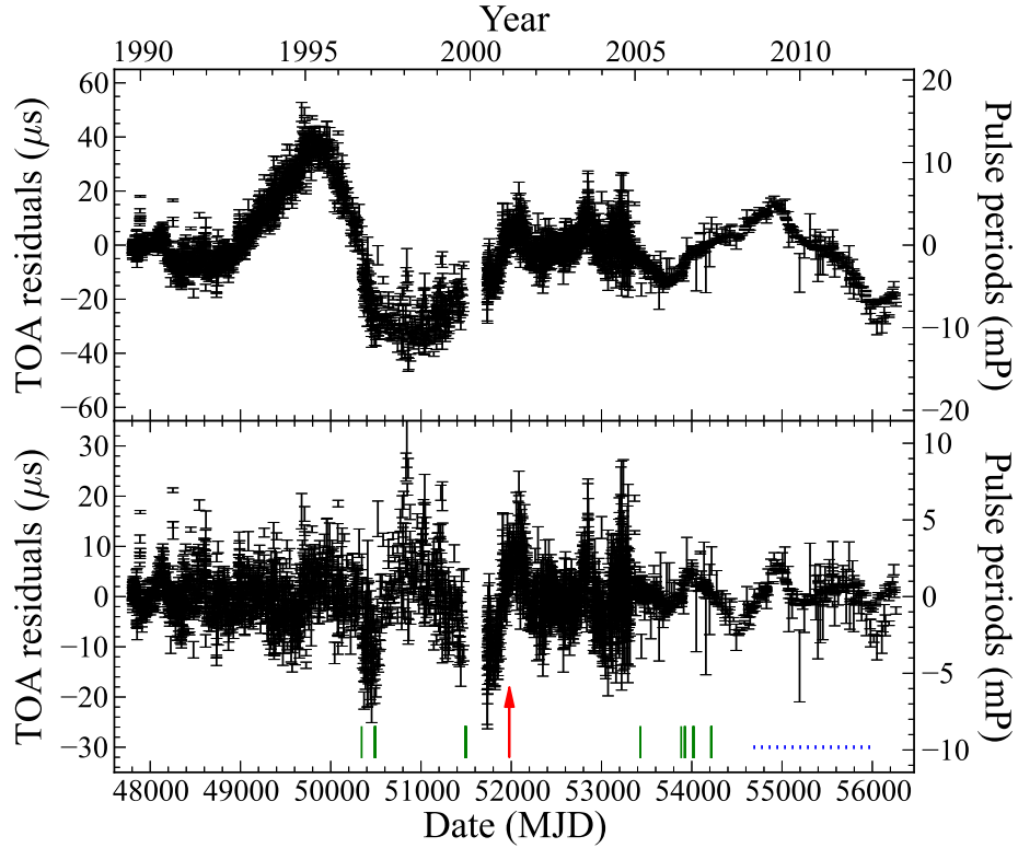
Fig. 2.— Timing residuals as a function of time, for the model given in Table 1 (upper panel), and after whitening of the residuals using eight harmonically related sinusoids (lower panel). The arrow (red in the online version) indicates the epoch of the glitch of PSR B1821–24, vertical lines (green in the online version) denote the epochs of the X-ray observations considered in this article, and the dashed horizontal line (blue in the online version) shows the Fermi LAT observation interval described in Section 3.3.
