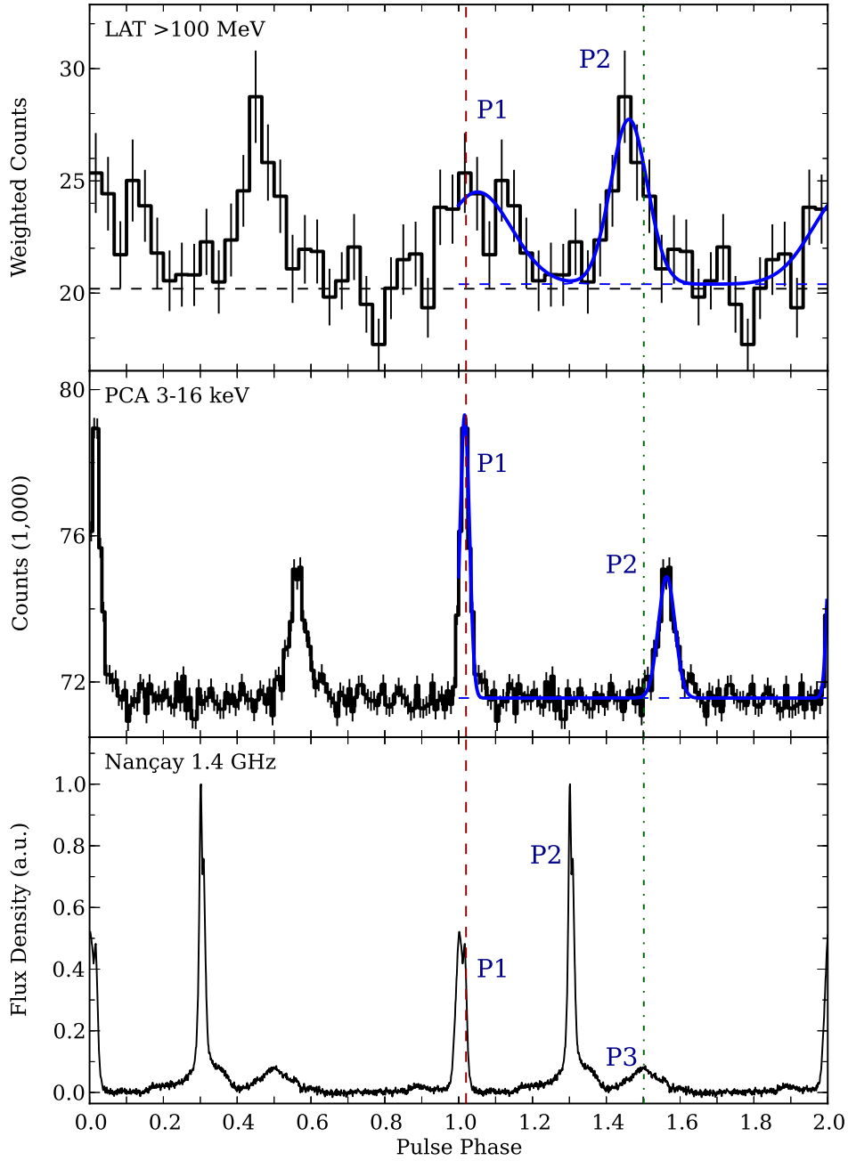
Fig. 5.— Folded light curves of PSR B1821–24, from top to bottom: \geq 100 MeV, 3 to 16 keV, and 1.4 GHz. The light curves are shown over two rotations for clarity, the solid (blue in the online version) lines over the second rotation in the top two panels are the best-fit light curve shapes. The dashed (red in the online version) vertical line indicates the approximate phase from which giant pulses have been observed. The dot-dash (green in the online version) vertical line indicates the center of P3 in the radio profiles.
