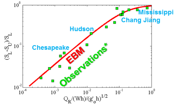
Figure 3 The points are observations in 13 estuaries regenerated from Geyer (2010), the solid line is the EBM solution.
