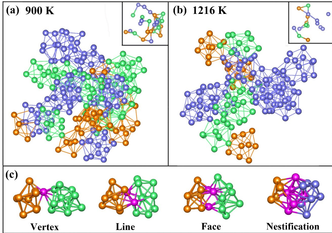
Fig. 5. Distribution of Z9 (orange clusters) 、 Z10 ( green ones ) and Icosahedron (blue ones) clusters in \text{Pd}_{82}\text{Si}_{18} at different temperature (a) 900 K, (b) 1216 K. (c) Connection way of different clusters, and pink ones are the sharing atoms.
