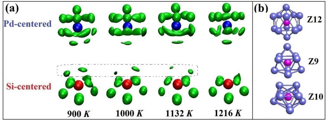
Fig. 3 (a) The results of the collective alignment for liquid \text{Pd}_{82}\text{Si}_{18} alloy at different temperatures. Clusters in the upper panel stand for the Pd-centered (blue) ones and those in the lower panel represent the Si-centered (red) ones. The size of each ball represents the probability of atoms of a cluster in this position. (b) Standard Z12, Z9 and Z10 cluster.
