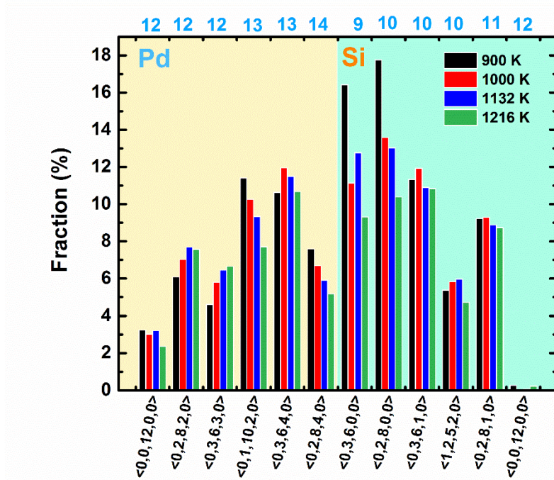
4 5 Fig. 4. The distributions of Voronoi indices for liquid \text{Pd}_{82}\text{Si}_{18} alloy at different 6 temperatures.
