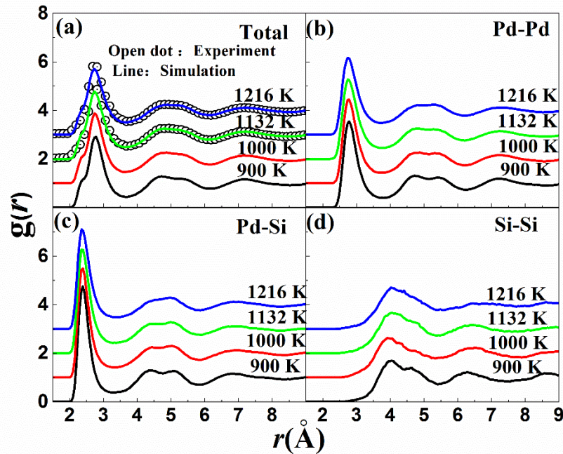
14 15 Fig. 1. The calculated total and partial pair correlation functions of liquid \text{Pd}_{82}\text{Si}_{18} alloy at 16 different temperatures. The solid lines and open dots represent calculated and 17 experimental, g(r) , respectively. The curves are shifted vertically as indicated by the 18 figures.
