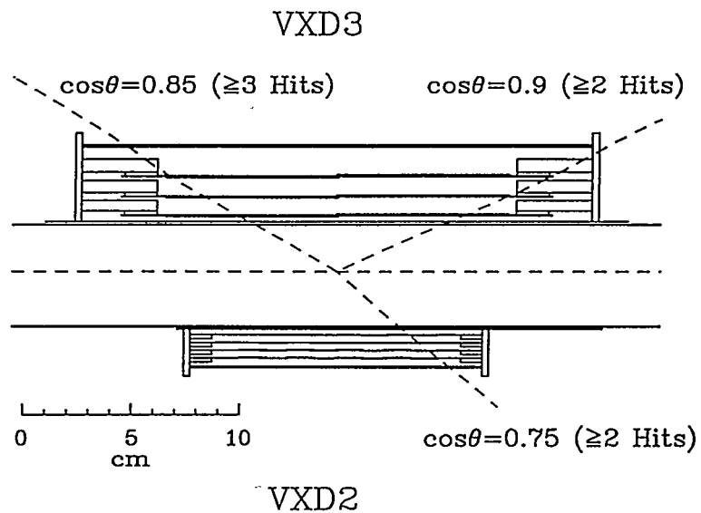
Figure 4. Comparison of VXD2 and VXD3 RZ profiles showing beam pipe, beryllium support structure, ladders, and CCDs.
