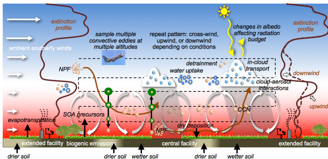
Figure 1. Schematic diagram depicting land-atmosphere, boundary-layer, and aerosol processes that influence the lifecycle of shallow convective clouds.
