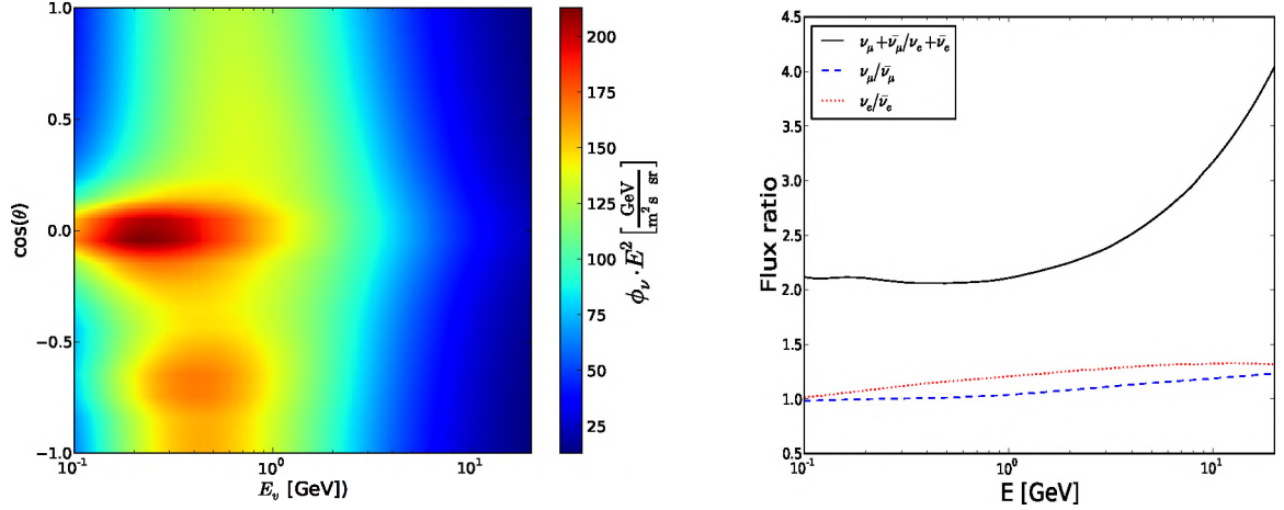
Figure 7-1: The differential ( \nu_\mu + \bar{\nu}_\mu ) flux density multiplied with E^2 versus energy and zenith angle (left) and flux ratios of different flavors versus energy averaged over all zenith angles (right).
