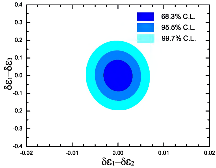
Figure 12-5: The experimental constraints on the generic NSI parameters \delta\epsilon_1 - \delta\epsilon_2 and \delta\epsilon_1 - \delta\epsilon_3 , where the true values are fixed at \delta\epsilon_1 - \delta\epsilon_2 = \delta\epsilon_1 - \delta\epsilon_3 = 0 . [450] The NH is assumed for illustration.
