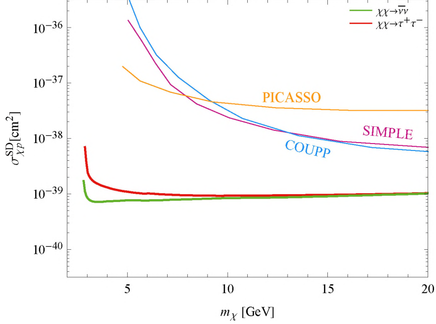
Figure 11-3: The JUNE 2\sigma sensitivity in 5 years to the spin-dependent cross section \sigma_{\chi p}^{\text{SD}} in 5 years. The constraints from the direct detection experiments are also shown for comparison.
