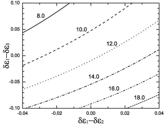
Figure 12-4: The iso- \Delta\chi^2 contours for the MH sensitivity as a function of two effective NSI parameters \delta\epsilon_1 - \delta\epsilon_2 and \delta\epsilon_1 - \delta\epsilon_3 . [450] The NH is assumed for illustration.
