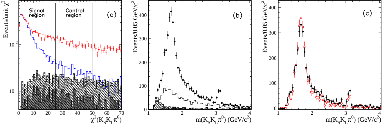
FIG. 3: (a) The four-constraint \chi^2 distributions for data (points) and MC-simulated K_S^0 K_L^0 \pi^0 \gamma events (open histogram). The shaded, cross-hatched, and hatched areas represent the simulated backgrounds from non-ISR q\bar{q} , ISR \phi , and ISR \phi\eta events, respectively. (b) The K_S^0 K_L^0 \pi^0 invariant mass distribution for data events in the signal region (points). The shaded, cross-hatched, and hatched areas represent the simulated contributions from non-ISR q\bar{q} , ISR \phi , and ISR \phi\eta events, respectively, while the open histogram represents the total background estimated from the control region. (c) The K_S^0 K_L^0 \pi^0 invariant mass distribution after background subtraction (points). The open circles represent the contribution from the resonant process e^+e^- \rightarrow K^*(892)^0 \bar{K}^0 + \text{c.c.} \rightarrow K_S^0 K_L^0 \pi^0 (see text).
