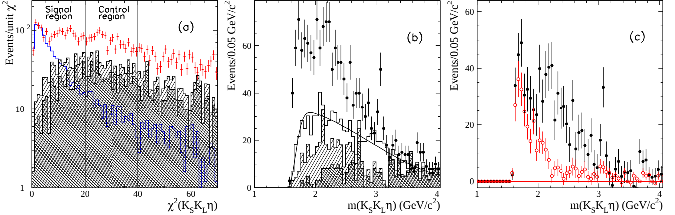
FIG. 9: (a) The four-constraint \chi^2 distributions for data (points) and MC-simulated K_S^0 K_L^0 \gamma \gamma events (open histogram). The cross-hatched and hatched areas represent the simulated backgrounds from non-ISR q\bar{q} events, and the sum of ISR K_S^0 K_L^0 \pi^0 , K_S^0 K_L^0 , and K_S^0 K_L^0 \eta events, respectively. (b) The K_S^0 K_L^0 \eta invariant mass distribution for data events in the signal region (points). The cross-hatched and hatched areas represent simulated backgrounds from non-ISR q\bar{q} and the sum of known ISR events, respectively, while the open histogram represents the total background, estimated from the control region. The curve shows the empirical fit used for background subtraction. (c) The K_S^0 K_L^0 \eta invariant mass distribution after background subtraction (points). The open circles represent the contribution from the resonant process e^+ e^- \rightarrow \phi \eta \rightarrow K_S^0 K_L^0 \eta (see text).
