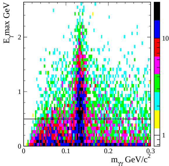
FIG. 2: Two-dimensional distribution of the higher cluster energy in a photon-candidate pair vs. the corresponding diphoton mass m_{\gamma\gamma} for all pairs of EMC clusters in K_s^0 K_L^0 \pi^0 \gamma events containing neither the ISR photon, the K_L^0 candidate, nor either photon in the \pi^0 candidate.
