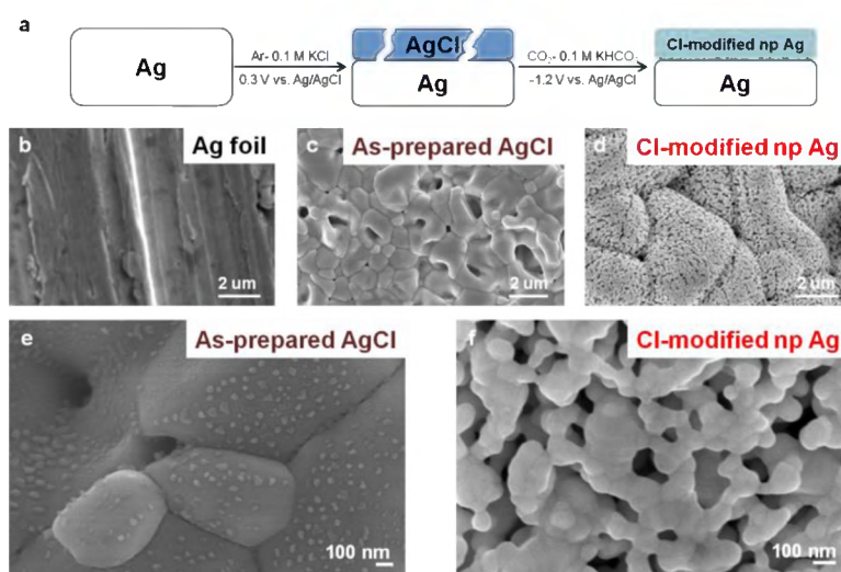
Figure 1. (a) Schematic illustration of the formation of as-prepared AgCl and in the presence of Cl. Scanning Electron Microscope (SEM) images of (b) untreated Ag foil, (c) as-prepared AgCl after 12 h oxidation, and (d) Cl-modified Ag. High-magnification SEM images of (e) as-prepared AgCl after 12 h oxidation and (f) Cl-modified Ag.
