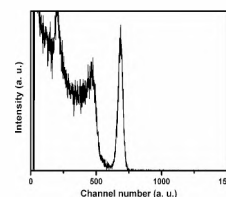
Figure 3. Pulse height spectra of \text{Cs}_2\text{LiCeCl}_6 crystal ^{137}\text{Cs} source.
