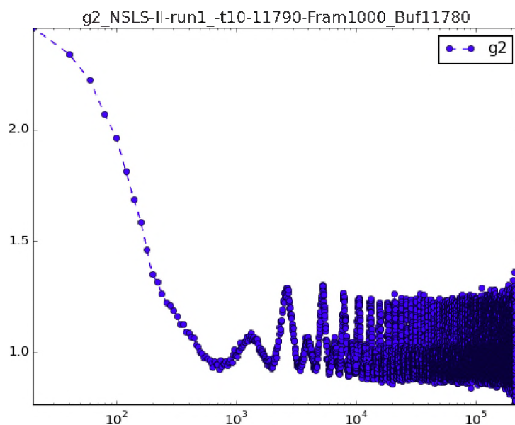
Figure 1. Plot of the pixel autocorrelation function, g_2 .
