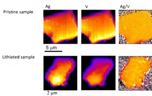
Figure 2. X-ray fluorescence images of Ag, V, and normalized Ag (i.e., Ag/V) from pristine and lithiated \text{Ag}_2\text{VO}_2\text{PO}_4 samples.
