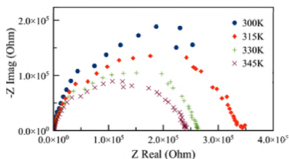
Figure 3. Electrical impedance spectra for PEO thin film devices at different temperatures.
