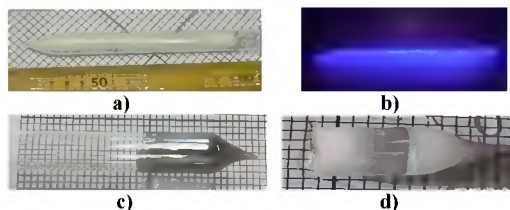
Figure 1. a) As-grown ingot (12-mm diameter), b) UV-light excited ingot, c) semi-transparent carbon coated ampoule, and, d) as-grown ingot (22-mm diameter).
