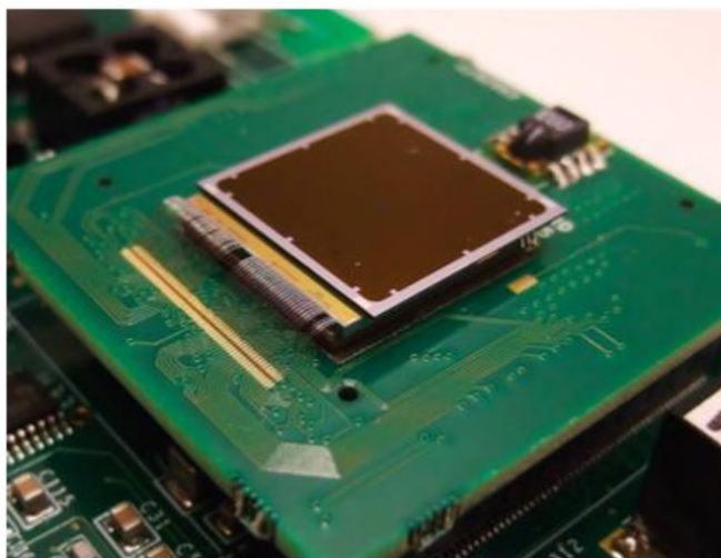
(a) The new sensor in TimepixCam.
