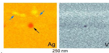
Figure 3. Ag clusters induced by X-ray beam.
