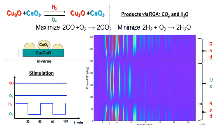
Figure 1. Oxidation-reduction of \text{Cu}_{60}\text{Ce}_{40} in a \text{H}_2/\text{O}_2 flow at 250^\circ\text{C} in a \text{CO}/\text{O}_2 stream.
