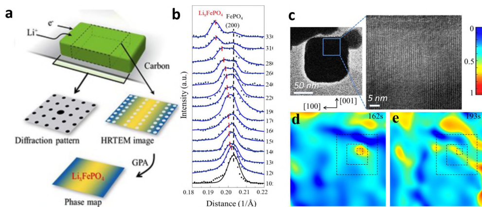
Figure 2. Real time tracking Li intercalation in a single LFP nanoparticle using a new in situ cell. (a) Schematic illustration of the setup. (b) Intensity profile of the electron diffraction recorded from a single LFP particle. (c) Bright-field and high-resolution TEM images of a single LFP particle selected for this study. (d, e) Maps of local Li concentration within the LFP particle at intermediate lithiated states.
