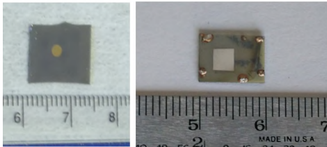
Figure 1. B_{12}As_2 thin-film detectors produced by E-beam evaporation (left) and CVD process (right).
