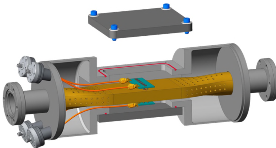
Figure 2. Assembly drawing of the proposed eRHIC time and space resolving BPM as adapted to the geometry of the ATF.
