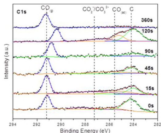
Figure 1. Preliminary AP-XPS experiments obtained at the ALS for the exposure of TiO x /Au(111) to ~0.1 Torr of CO.
