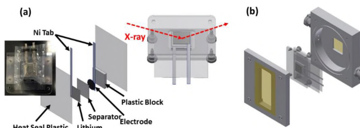
Figure 1. (a) In situ plastic pouch cell schematic and (b) in situ enclosure to ensure the pouch cell is measured under inert atmosphere.
