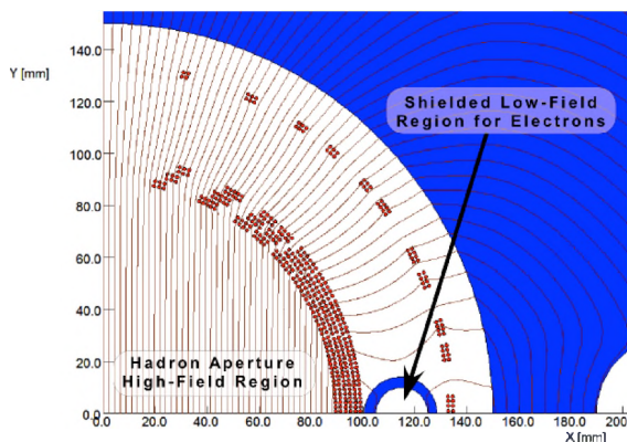
Figure 1. eRHIC IR dipole sweet spot concept.
