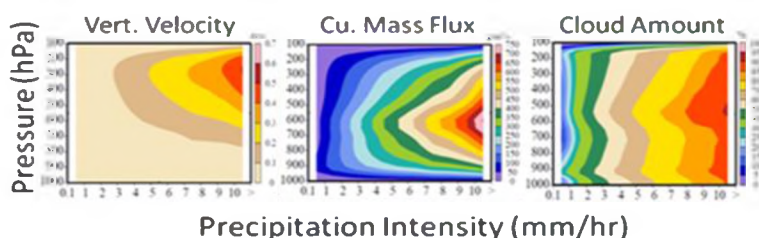
Figure 1. Vertical velocity, cumulus mass flux and cloud amount from WRF simulation as a function precipitation intensity. Companion CAM simulation has weaker vertical velocity and weaker cumulus activities peaked at much higher altitudes, suggesting weaker entrainment and lack of anvil representation.
