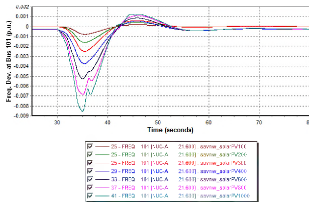
Figure 1. Impacts of different penetration levels of PV generation on the inertial response.
