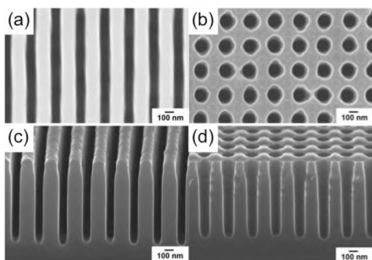
Figure 1. Topdown (a, b) and cross-sectional (c, d) Scanning Electron Microscope images of silicon templates with grating (a, c) and pore (b, d) geometries.
