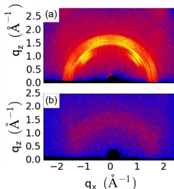
Figure 2. GIWAXS spectra of (a) highly crystalline PEO film, and (b) PEO film confined within nanoscale pores.
