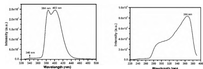
Figure 2. Left: Emission and Right: excitation spectrum.
