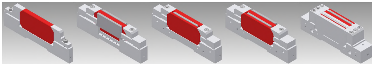
Figure 3. Computer Aided Design models of modules (left to right: M, PMP, MPN, PMPN, T) constituting the SAGIVU magnet system. Such models and fabrication drawings were produced for 3 SAGIVU segments for the Low-Beta straight section of NSLS-II and for 1 segment for the High-Beta straight section. This set includes 20 different modules and more than 100 individual fabrication drawings. All drawings and technical specifications are currently “released” and prepared for a “build-to-print” type procurement procedure.
