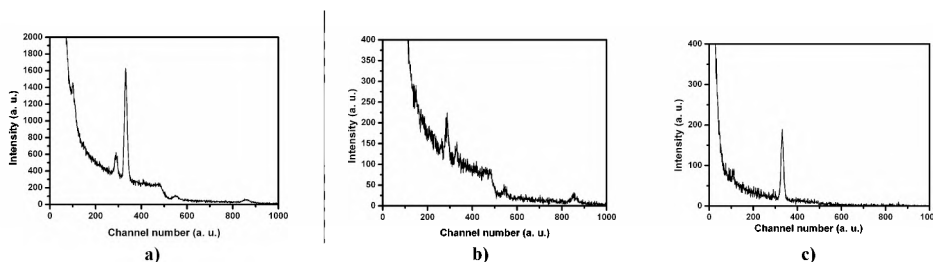
Figure 4. Pulse-height spectra for an Am-Be source; a) open source, b) window blocked with cadmium sheet and c) the window blocked with a 2-inch-thick lead shield.
