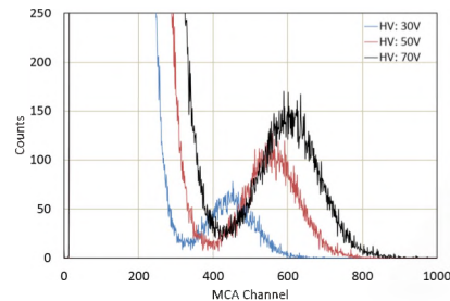
Figure 3. ^{241}Am spectra obtained with a B_{12}As_2 thin-film detector.
