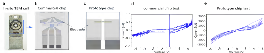
Figure 1. (a) Optical image of the in situ TEM cell. Electrode diagrams for (b) commercial chip and (c) prototype chip. Electrochemical measurements of water dissociation using (d) commercial chip and (e) prototype chip.
