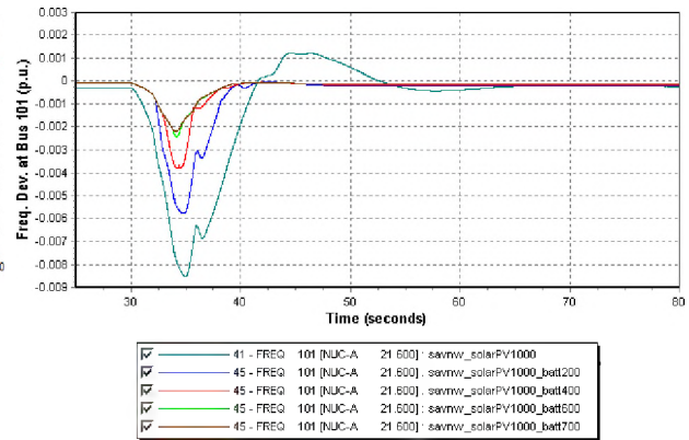
Figure 2. Performance of different capacity of battery systems on the inertial response.
