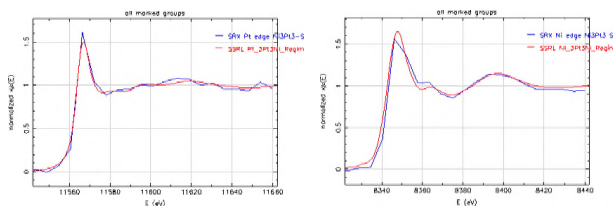
Figure 2. Spectroscopy + imaging of bimetallic catalysts in operando conditions Pt L 3 edge (left) and Ni K edge (right) data in Pt 3 Ni 3 /SiO 2 nanocatalysts (J. Chen's group). Data acquisition time at SRX: 5-10 min (blue). Similar data at X27A (red): 2 hours of averaging!
