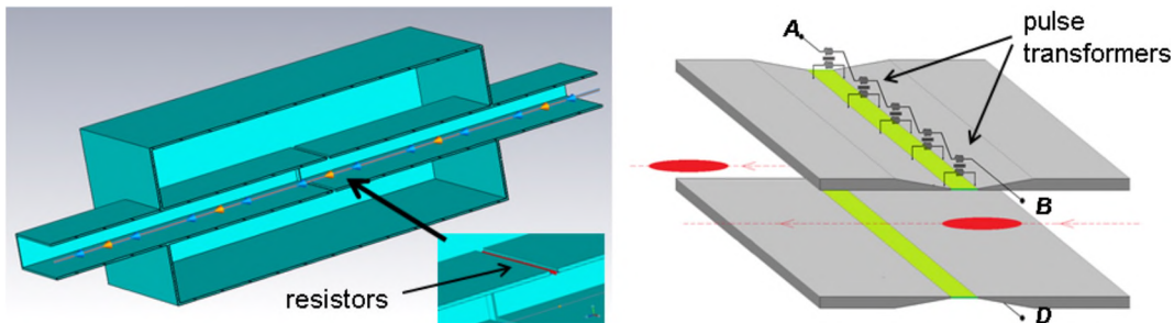
Figure 1. Conceptual view of the BPM showing beam traversing the small gap spanned by resistors (left) which are read out using pulse transformers (right).
