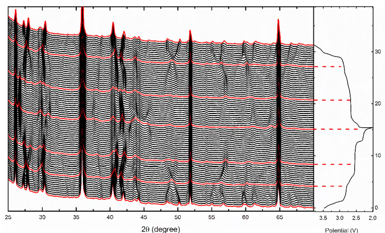
Figure 2. In situ XRD measurements on \text{LiV}_3\text{O}_8 electrode using laboratory based diffractometer. Data was continuously collected over a complete discharge and charge of the \text{LiV}_3\text{O}_8 electrode.
