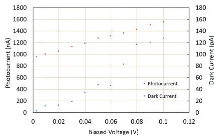
Figure 2. I-V measurement results from a B_{12}As_2 sample.
