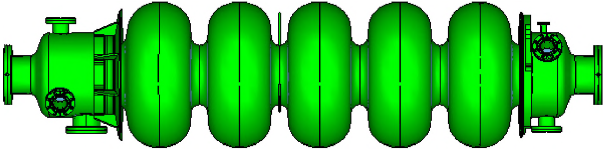
Figure 1. 5-cell 650 MHz eRHIC cavity.
