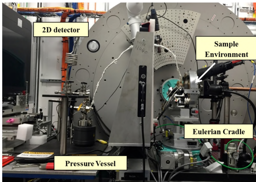
Figure 1. The in situ cell at XPD in an in situ corrosion study.
