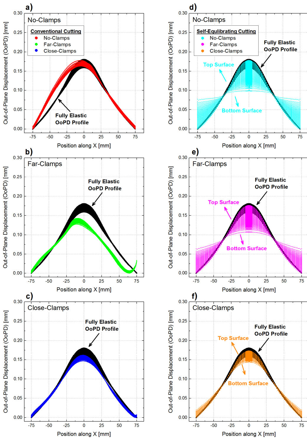
Fig. 4: Predicted out-of-plane displacement (OoPD) for conventional (a-c) and self-equilibrating (d-f) cutting strategies, under the clamping configurations shown in Fig. 3, compared to the fully elastic (ideal) OoPD profile (black).
