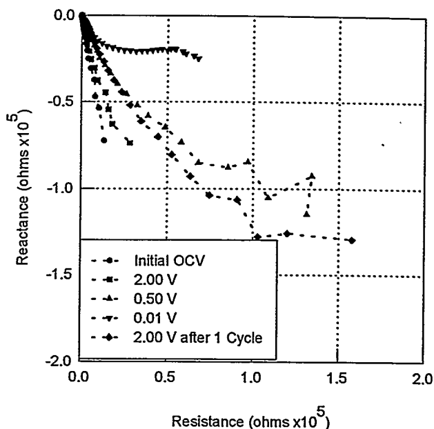
Figure 5. Complex-impedance spectra of glassy carbon at OCV as a function of applied potential during first reduction.
