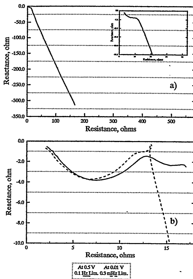
Figure 3. Complex-impedance spectra of 700°C PMAN carbon as a function of potential during the 17th intercalation cycle. a) At 2 V; b) at 0.5 V and 0.01 V.
