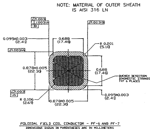
Fig. 3 TPX PF-6 & PF-7 Conductor
