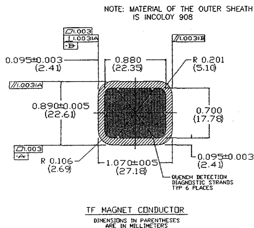
Fig. 1 TPX TF Conductor
