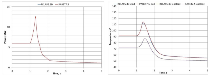
Figure 13 Results Calculated for EXP Transient
