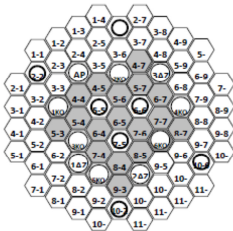
Figure 2 LEU Core Configuration for Cycle 1
