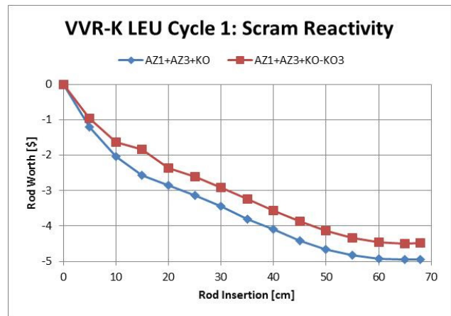
Figure 5 Scram Reactivity as Function of Rod Insertion
