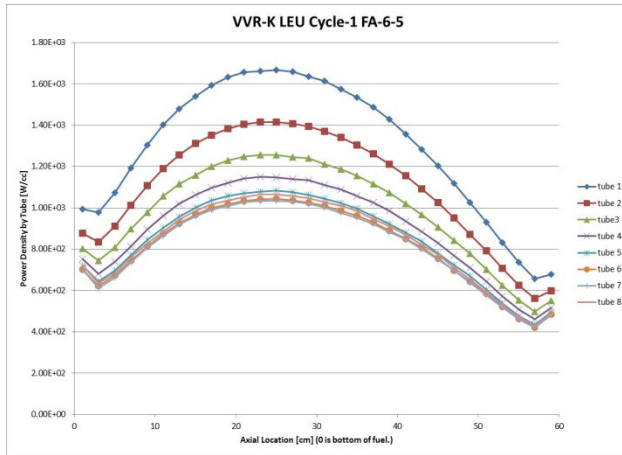
Figure 6 Axial Variation of Power Density by Tube for Peak Power FA in Cycle 1
