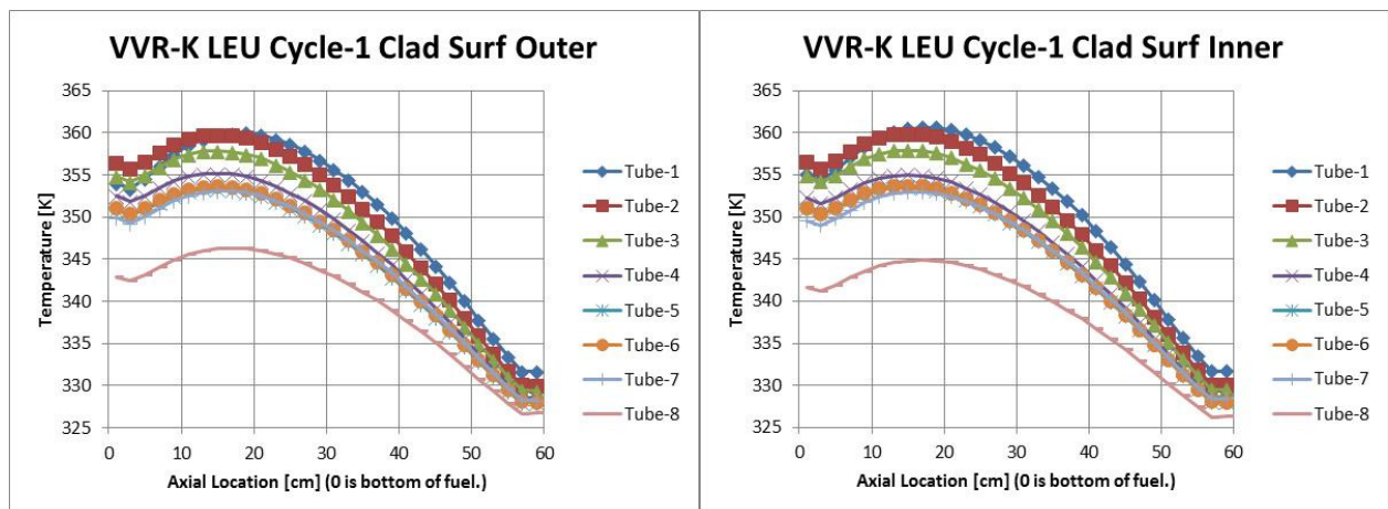
Figure 8 Outer Clad Surface Temperature Calculated using RELAP5
