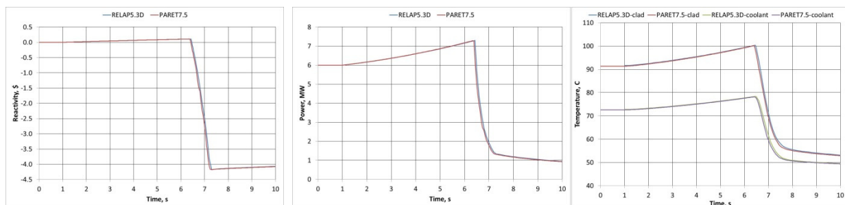
Figure 10 Results Calculated for KO Transient
