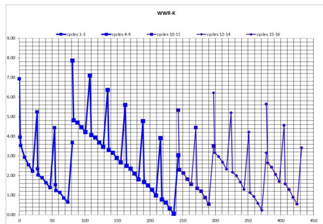
Figure 3 Excess Reactivity [%] vs. Time [full power days]
