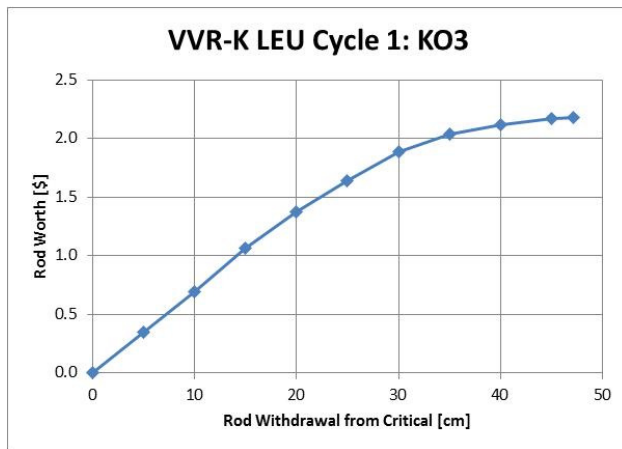
Figure 4 KO3 Rod Worth as Function of Withdrawal
