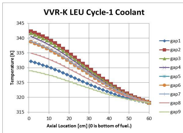
Figure 7 Coolant Temperature Calculated using RELAP5
