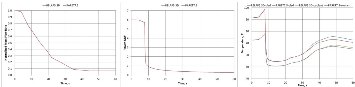
Figure 12 Results Calculated for LOOP Transient
