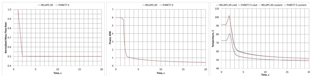
Figure 11 Results Calculated for BLADE Transient
