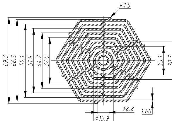
Figure 1 LEU Type FA-1 Fuel Assembly Geometry [1]
